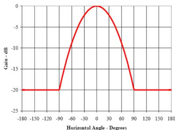
Figure 7.7.4-2 Simplified antenna pattern [ITU-R M.2135].
