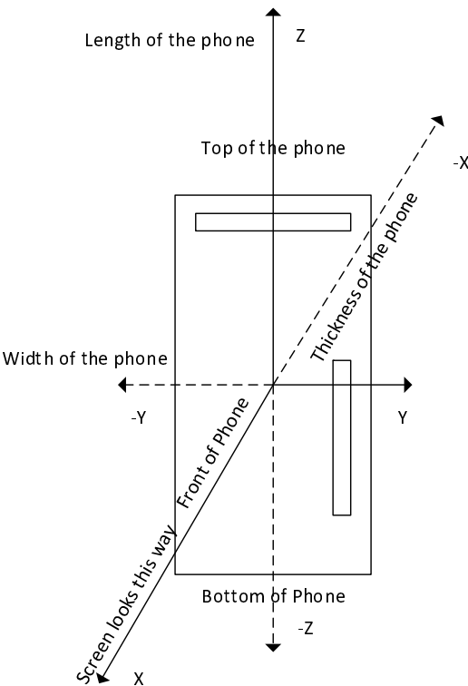
Figure E.2-1: Reference coordinate system and reference device orientation
