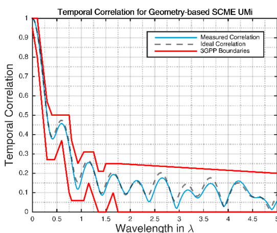
Figure 8.4.3-4b: Temporal correlation measurements of SCMe UMa and UMi for the RTS method with geometric implementation for System 2 with CE2 for Band 7
