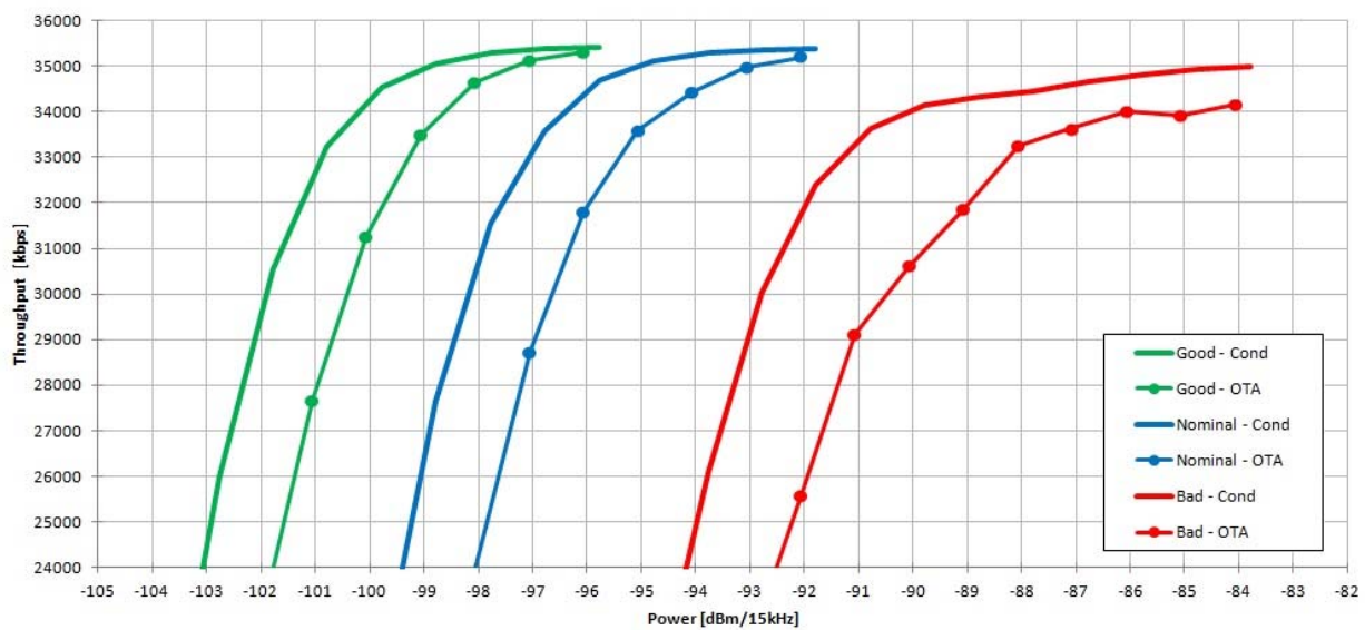
Figure 9.3.1.7.3-2: Proof of concept for the reverberation chamber and channel emulator methodology emulating the long delay spread high correlation channel model
