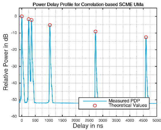
Figure 8.4.2-3b: SCMe UMA and UMi PDP verification measurement for the RTS method with correlation implementation (Jake's Doppler spectrum) for System 2 with CE2 for Band 7
