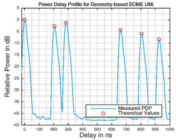
Figure 8.4.2-2a: SCMe UMA and UMi PDP verification measurement for the RTS method with geometric implementation for System 2 with CE2 for Band 13
