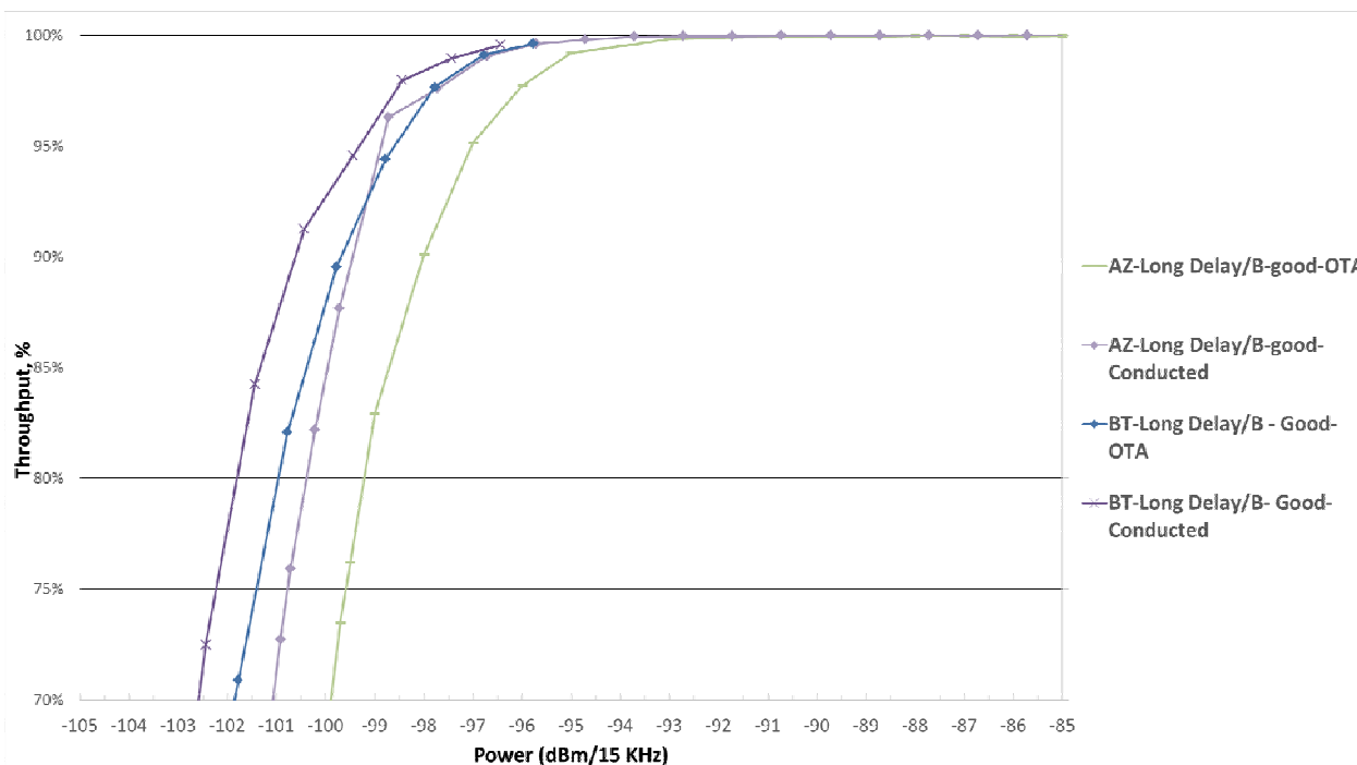
Figure 10.2.3-10: IL/IT results consistency for reverberation chamber methodology 2 (RC+CE) measurements implementing the Long Delay Spread High Correlation channel model with Good reference antenna only
