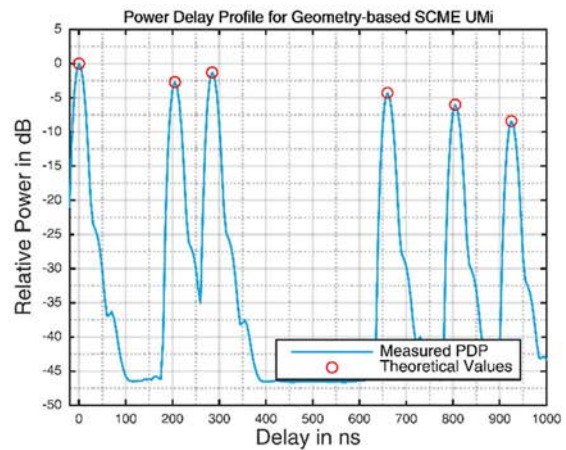
Figure 8.4.2-2b: SCMe UMA and UMi PDP verification measurement for the RTS method with geometric implementation for System 2 with CE2 for Band 7
