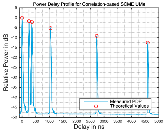
Figure 8.4.2-3a: SCMe UMA and UMi PDP verification measurement for the RTS method with correlation implementation (Jake's Doppler spectrum) for System 2 with CE2 for Band 13
