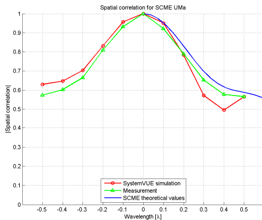
Figure 8.4.4-3: Band 13 spatial correlation measurements for the conducted two-stage method using correlation implementation of SCMe UMa and UMi with Jake's Doppler spectrum
