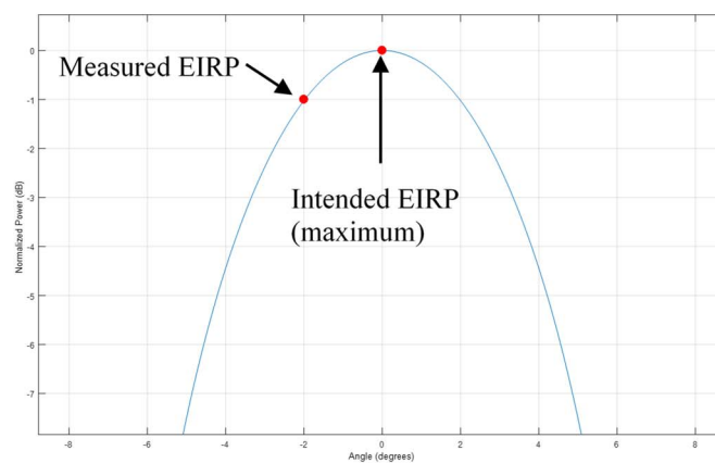
Figure 6.3.3-1: Angular misalignment
