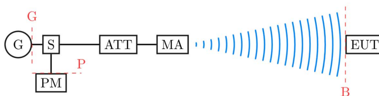
Figure 8.3.1.2-3: Measurement setup for receiver requirement measurement using a Power Meter
