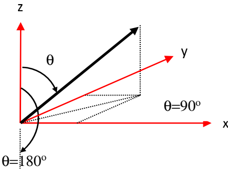
Figure 4-6: Another representation of θ angle (positive values only)
