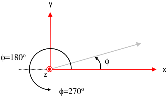
Figure 4-5: Another representation of the φ angle (positive values only)
