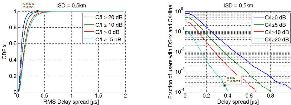
Figure 5.5.4.4-1: Urban environment with small microcells
