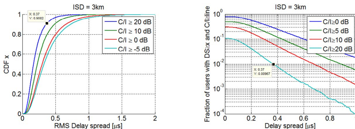
Figure 5.5.4.4-2: Urban environment with microcells
