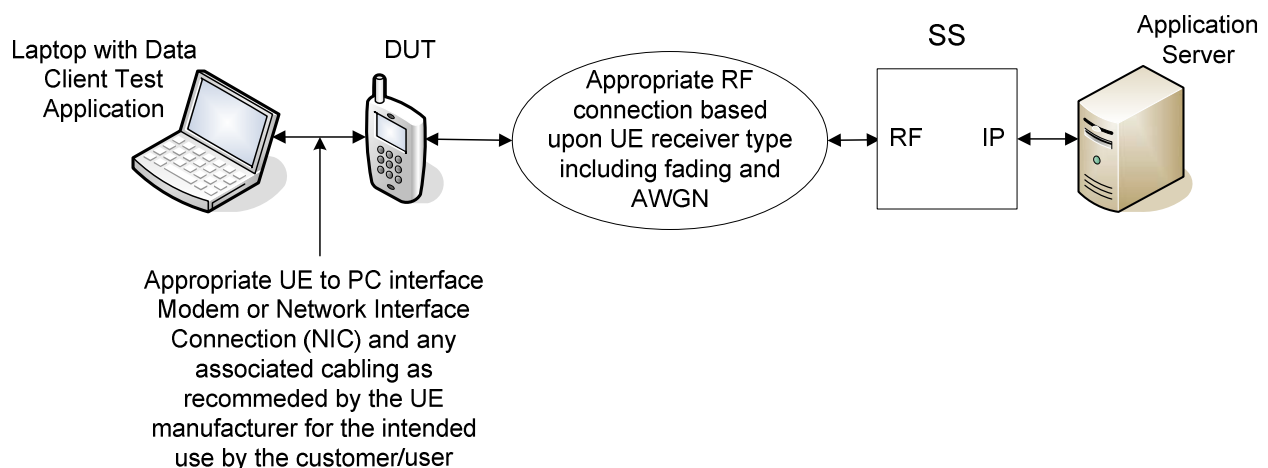
Figure C.2.1-1: UE Application Layer Data Throughput Connection Diagram for Tethered
