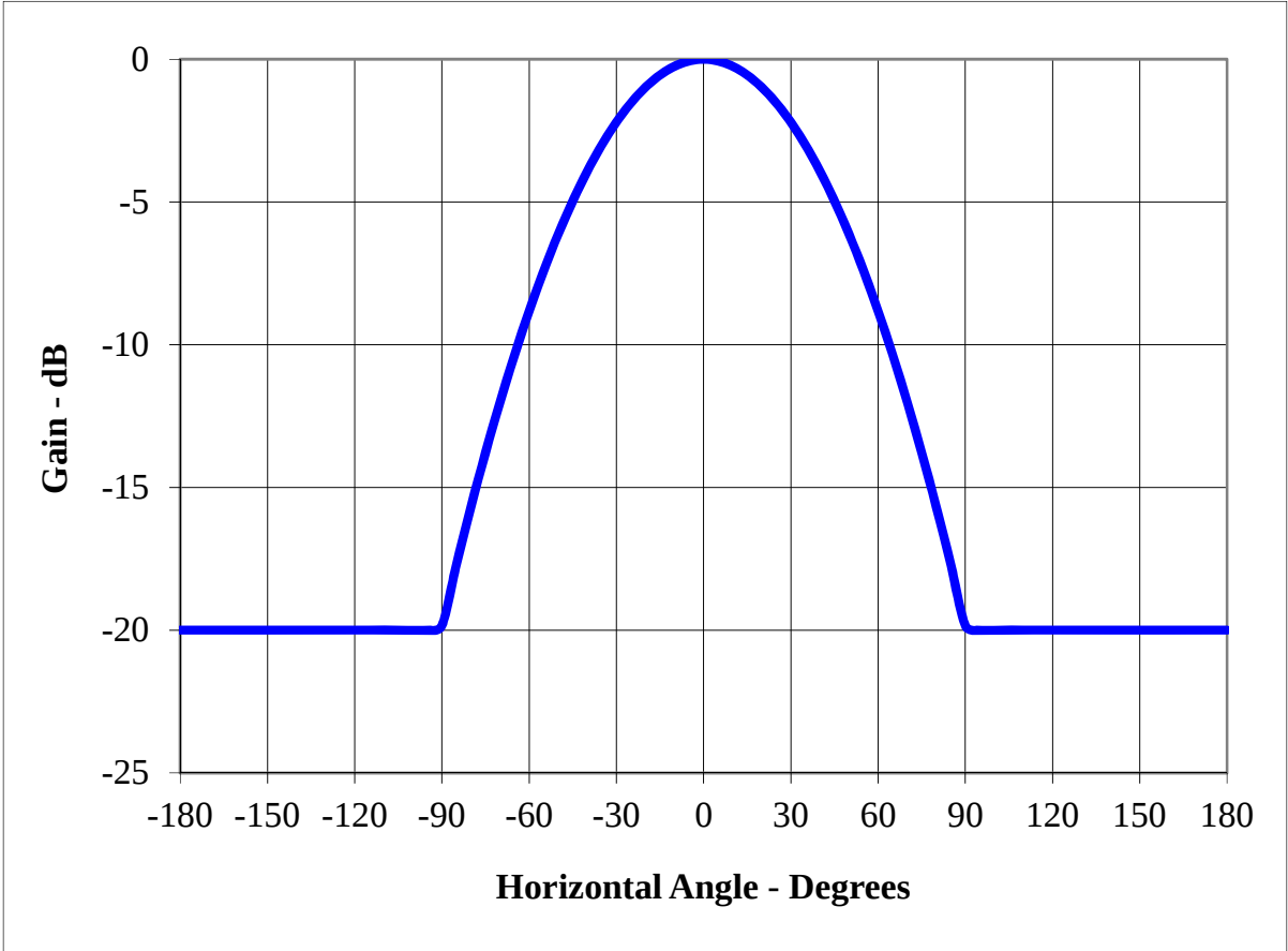
Figure 4.1: Antenna Pattern for 3-Sector Cells
