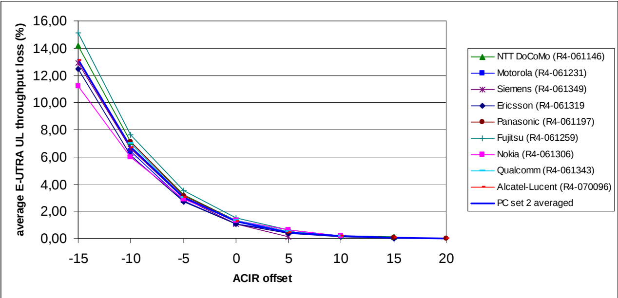
Figure 7.3d: Average E-UTRA uplink throughput loss for power control set 2
