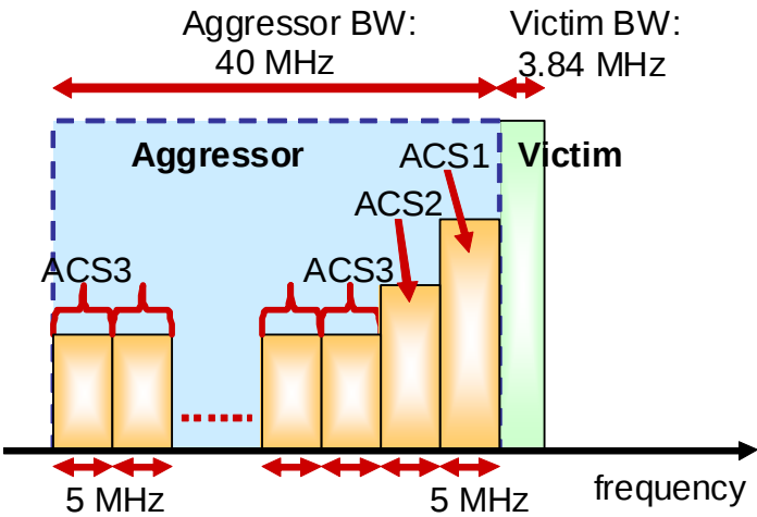
Figure 12.9 Downlink ACIR model for Scenario #3
