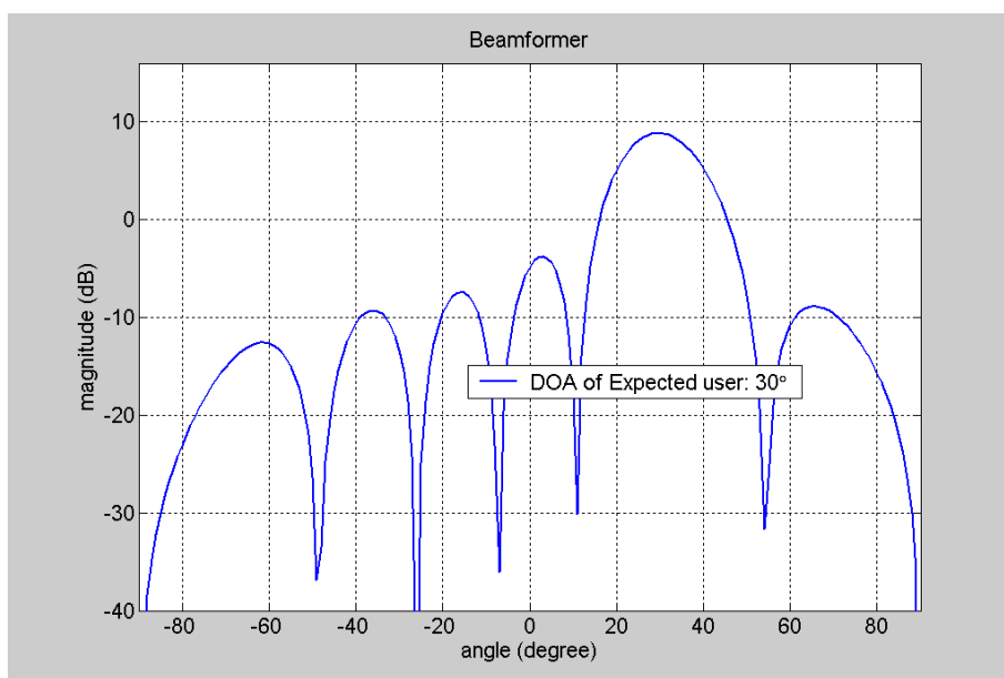
Figure B.2: 30^\circ beam forming pattern
