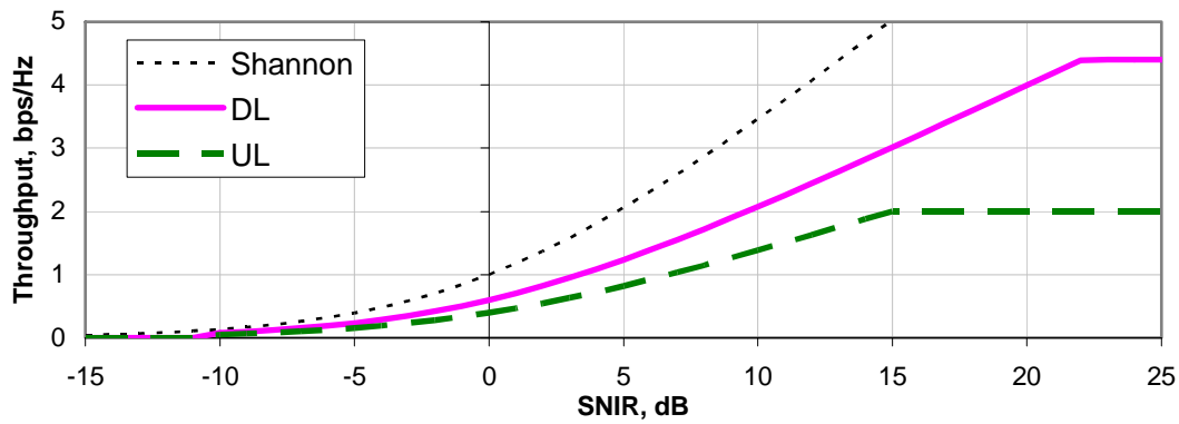
Figure A.1 Throughput vs SNR for Baseline E-UTRA Coexistence Studies
