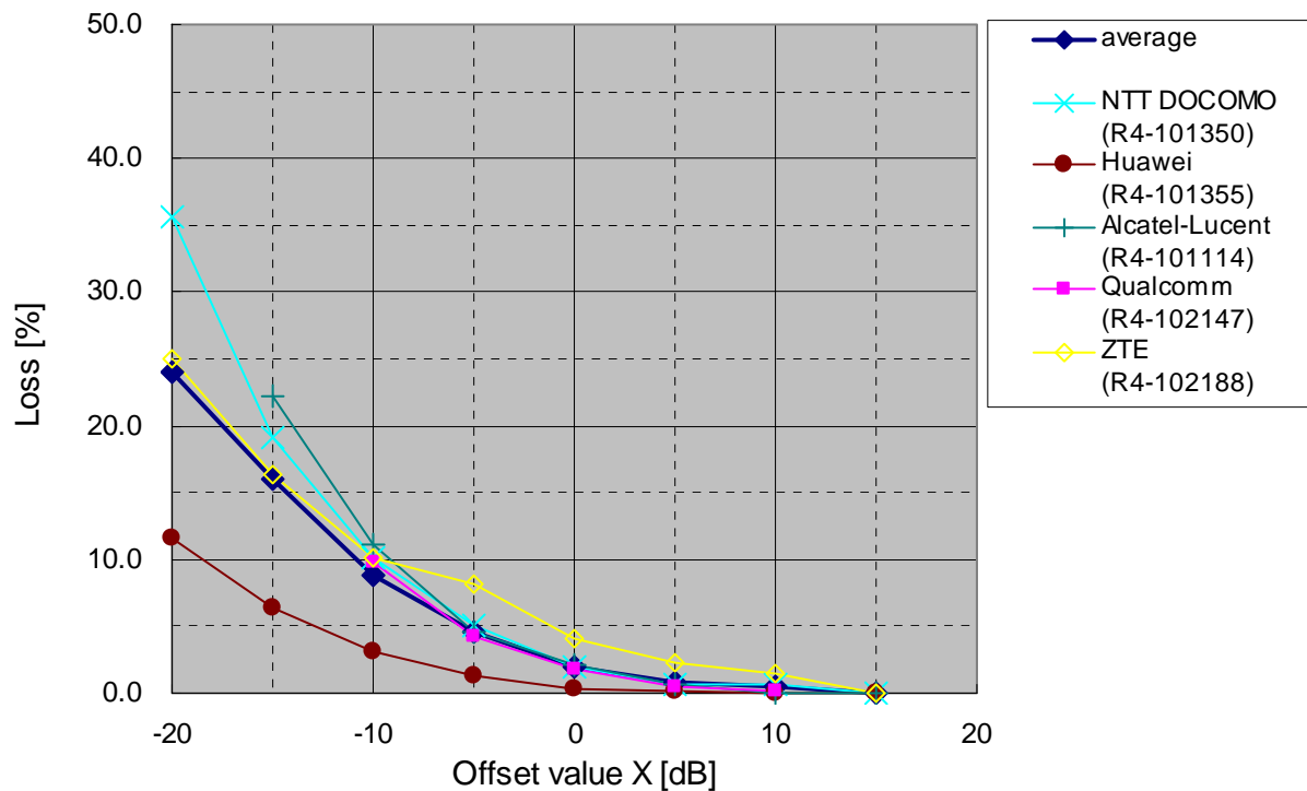
Figure 12.23 average 5 MHz UTRA downlink capacity loss
