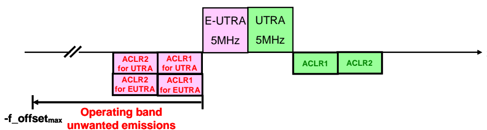
Figure 10.4: Unwanted emissions requirements for multi-carrier BS of E-UTRA and UTRA
