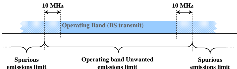
Figure 11.3 Defined frequency ranges for spurious emissions and operating band unwanted emissions
