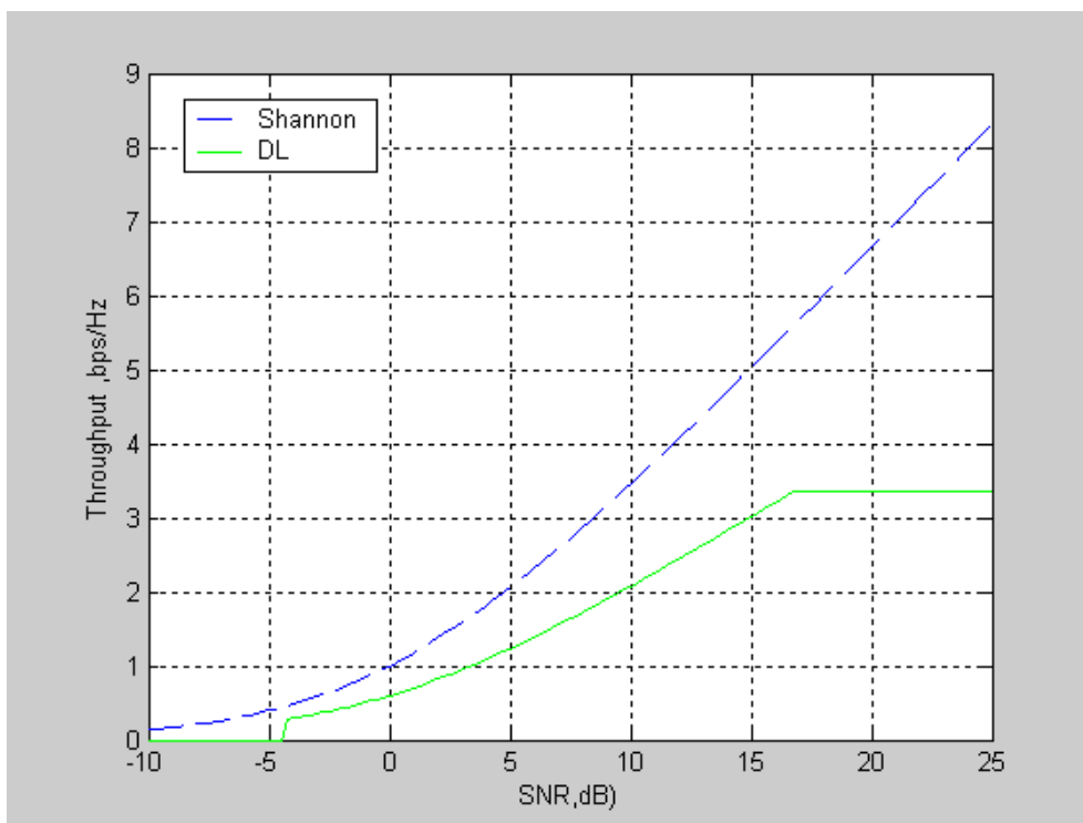
Figure A.8 Throughput vs SNR for Baseline E-UTRA Coexistence Studies for downlink
