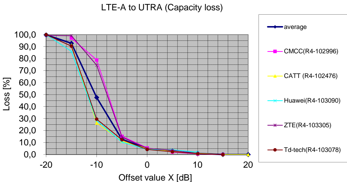
Figure 12.26 average 1.6 MHz UTRA downlink capacity loss
