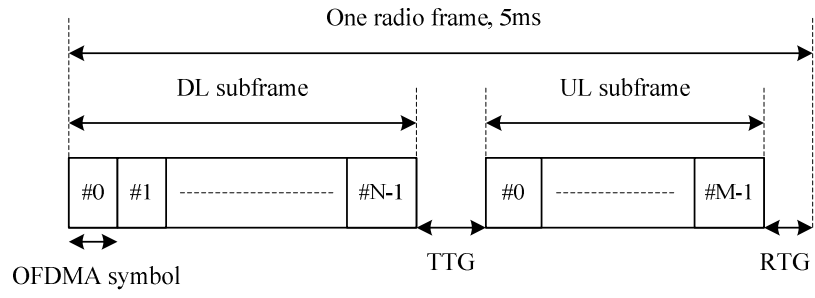
Figure B-2: Frame structure
