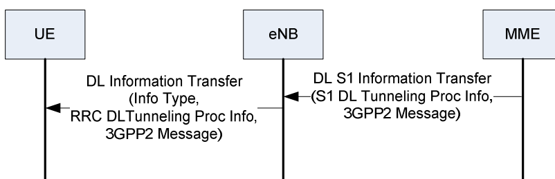
Figure 6.1-1 Downlink Direct Transfer
