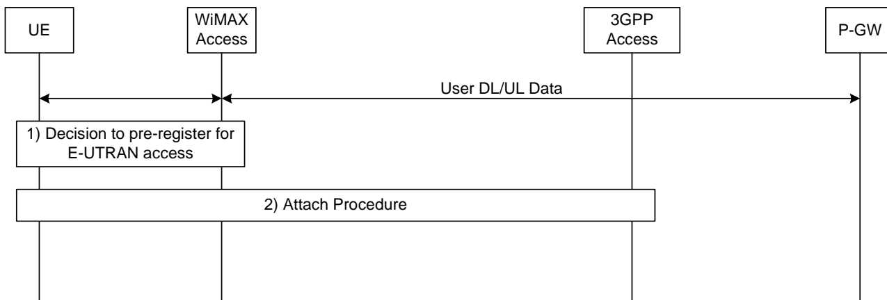
Figure 7.5-2 Pre-registration to the E-UTRAN
