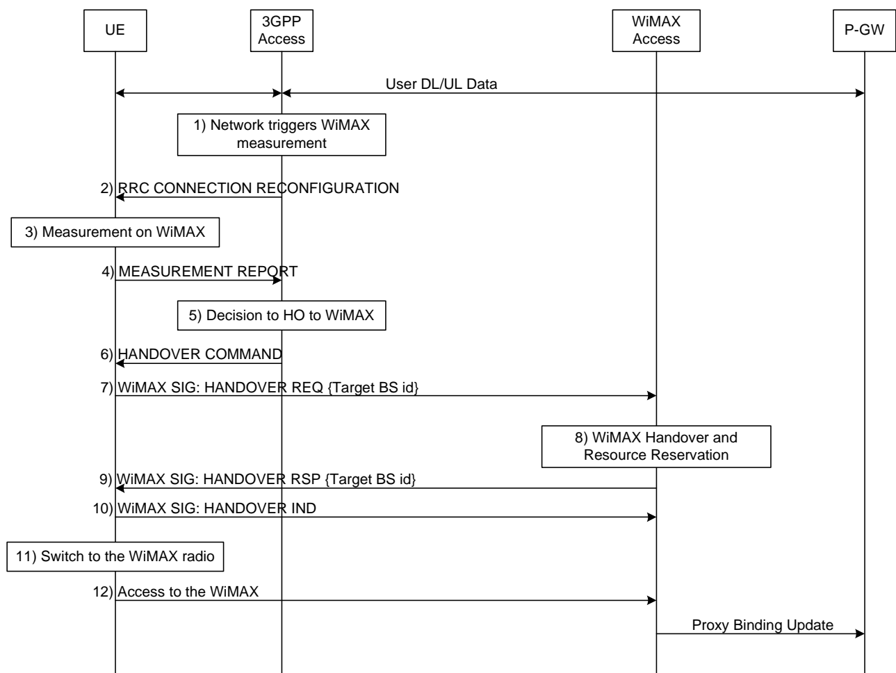
Figure 7.4-3 Optimized E-UTRAN to WiMAX Handover
