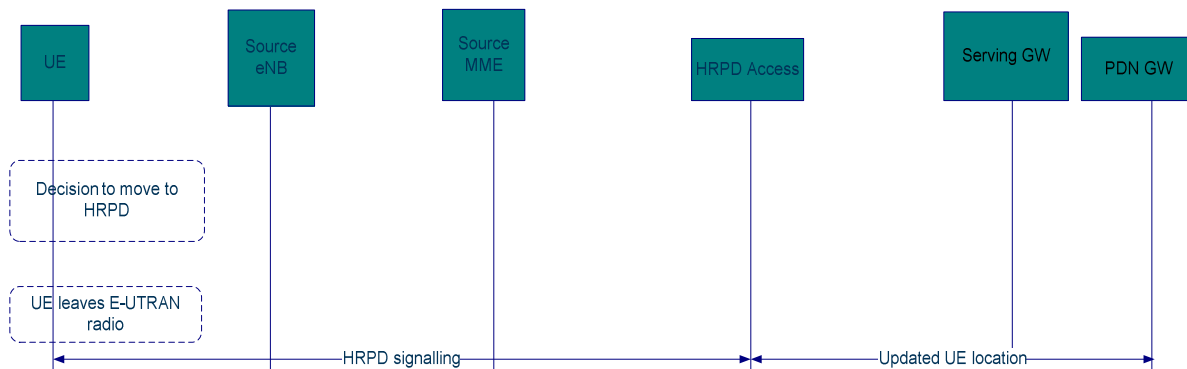
Figure 6.2-3 E-UTRAN to HRPD Cell Re-Selection
