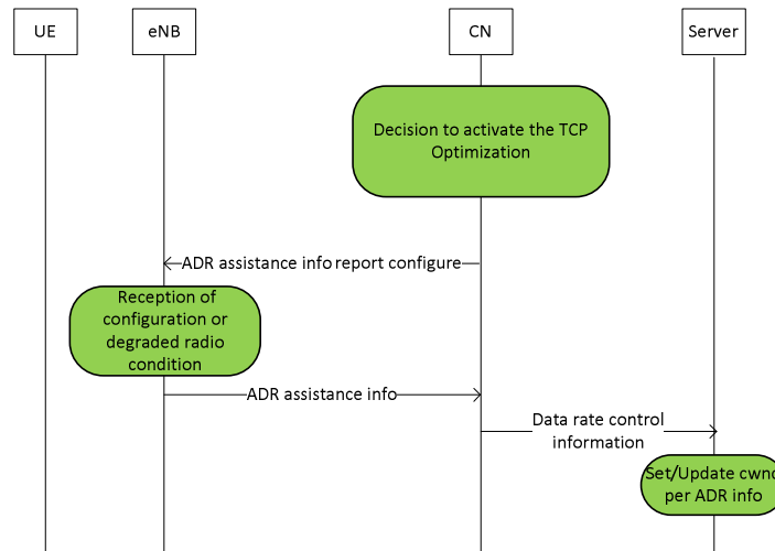
Figure 5.3.2-1: Network assisted radio-aware TCP solution
