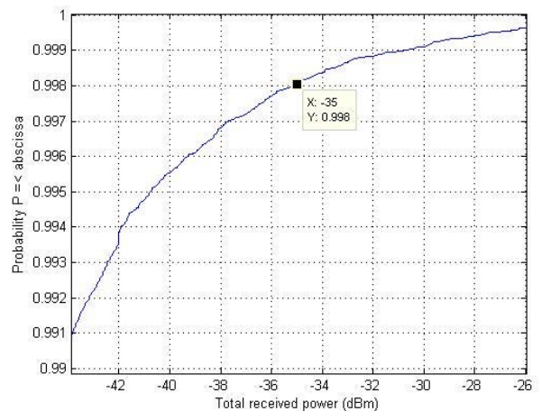
Figure 6.1.2.2.1-2 CDF of the total received blocking power (zoomed version), no UE blocking
