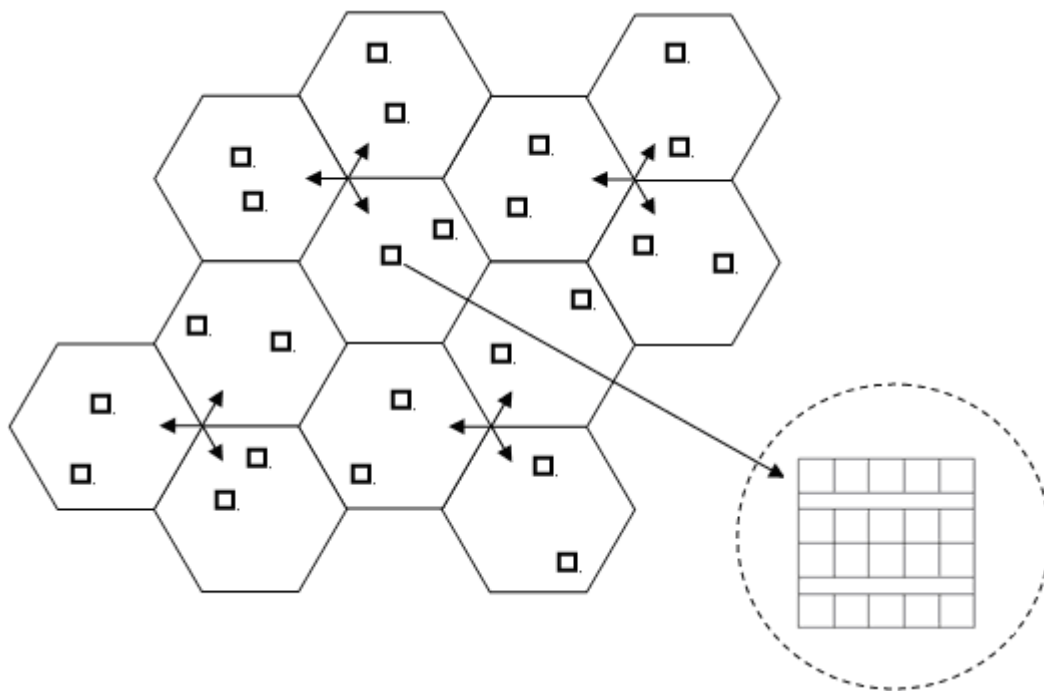
Figure 5.3.1.2-1. Macro-Pico deployment
