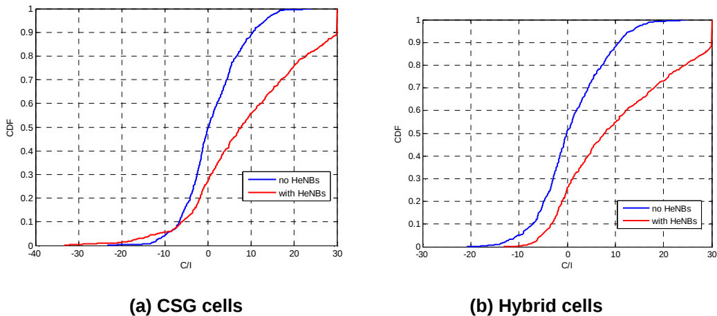
Figure 7.5.2-3 C/I for CSG cells and hybrid cells deployments with adaptive HeNB Tx power
