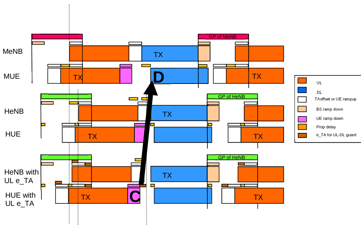
Figure 6.5-1 TDD HeNB Timing using Network Listening and Extra Timing Advance
