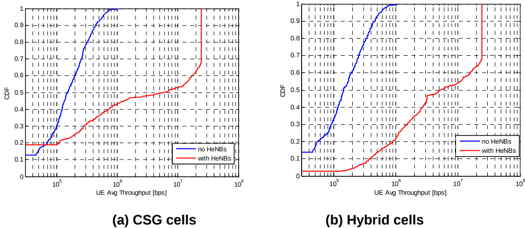
Figure 7.5.2-2 Throughput for CSG cells and hybrid cells deployments with 8 dBm HeNB Tx power
