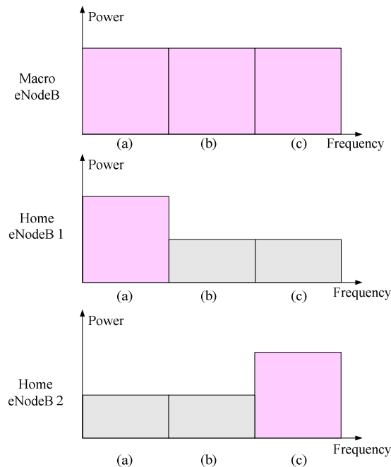
Figure 5.1-1 Frequency Partitioning
