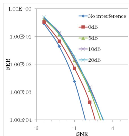
Fig. 7.4.1.1-3 4CCE PDCCH BLER with subband interference estimation
