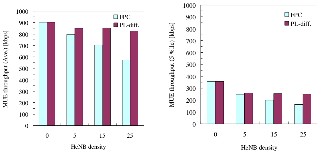
Figure 7.3.2.2.2-1: MUE throughput (Left: Average, Right: 5 percentile)
