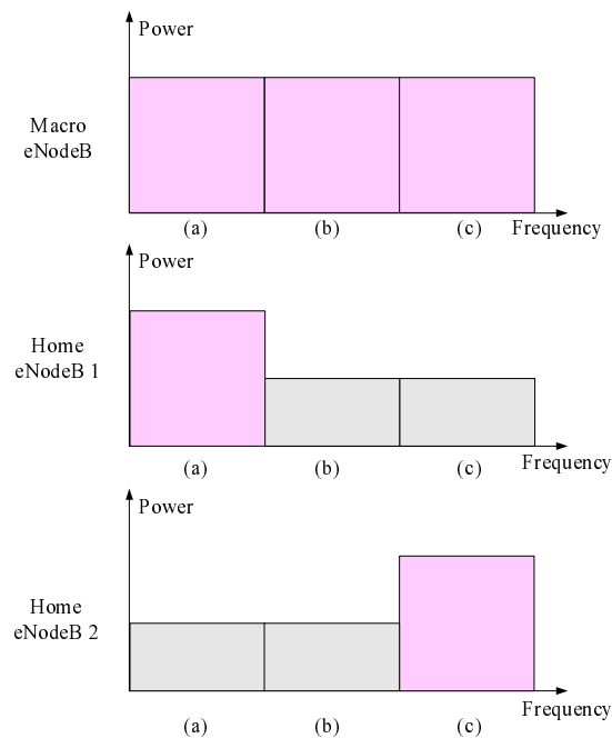
Figure 5.1-1 Frequency Partitioning
