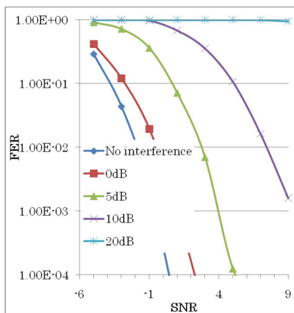
Fig. 7.4.1.1-2 CCE PDCCH BLER with wideband interference estimation
