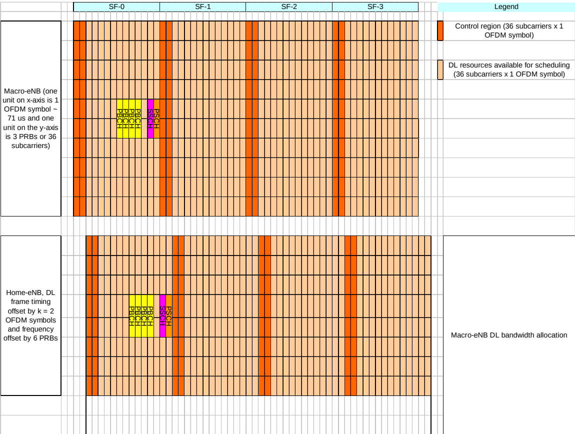
Figure 7.2.1.2 Time-shift HeNB frame timing by k = 2 OFDM symbols and offset the HeNB carrier by 6 PRBs (1.08 MHz) relative to macro-eNB timing and carrier respectively
