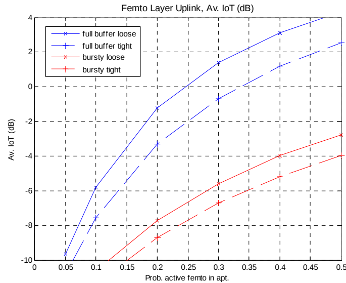
Figure 7.3.2.1.1.2-6: Femtocell Interference over Thermal
