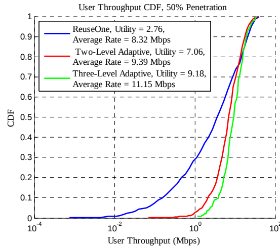
Figure 7.2.3.3: User throughput CDF for reuse one and adaptive resource coordination with 50% penetration
