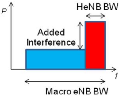
Fig. 7.2.1.2-1 Partial Bandwidth Coexistence
