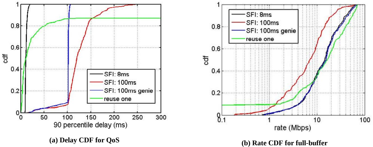
Figure 7.2.3.2 Delay and data rate CDF for mixed traffic with 50% penetration
