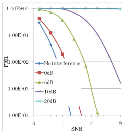
Fig. 7.2.1.4.2 4 CCE PDCCH BLER with wideband interference estimation
