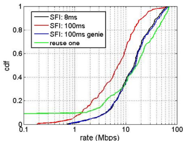
(b) Rate CDF for full-buffer
