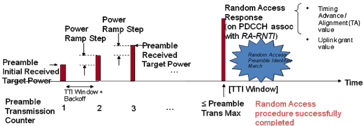
Figure 4.7.4.1.1-1: RACH Procedure
