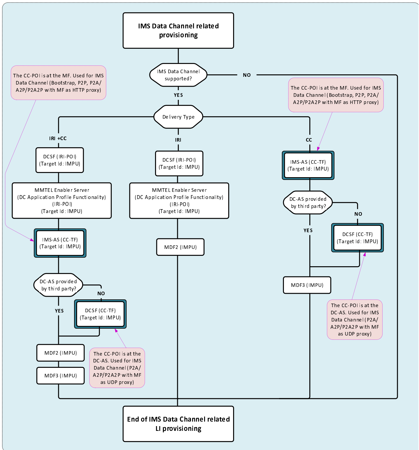
Figure 5.5.4.2.5-1: IMS Data Channel perspective
