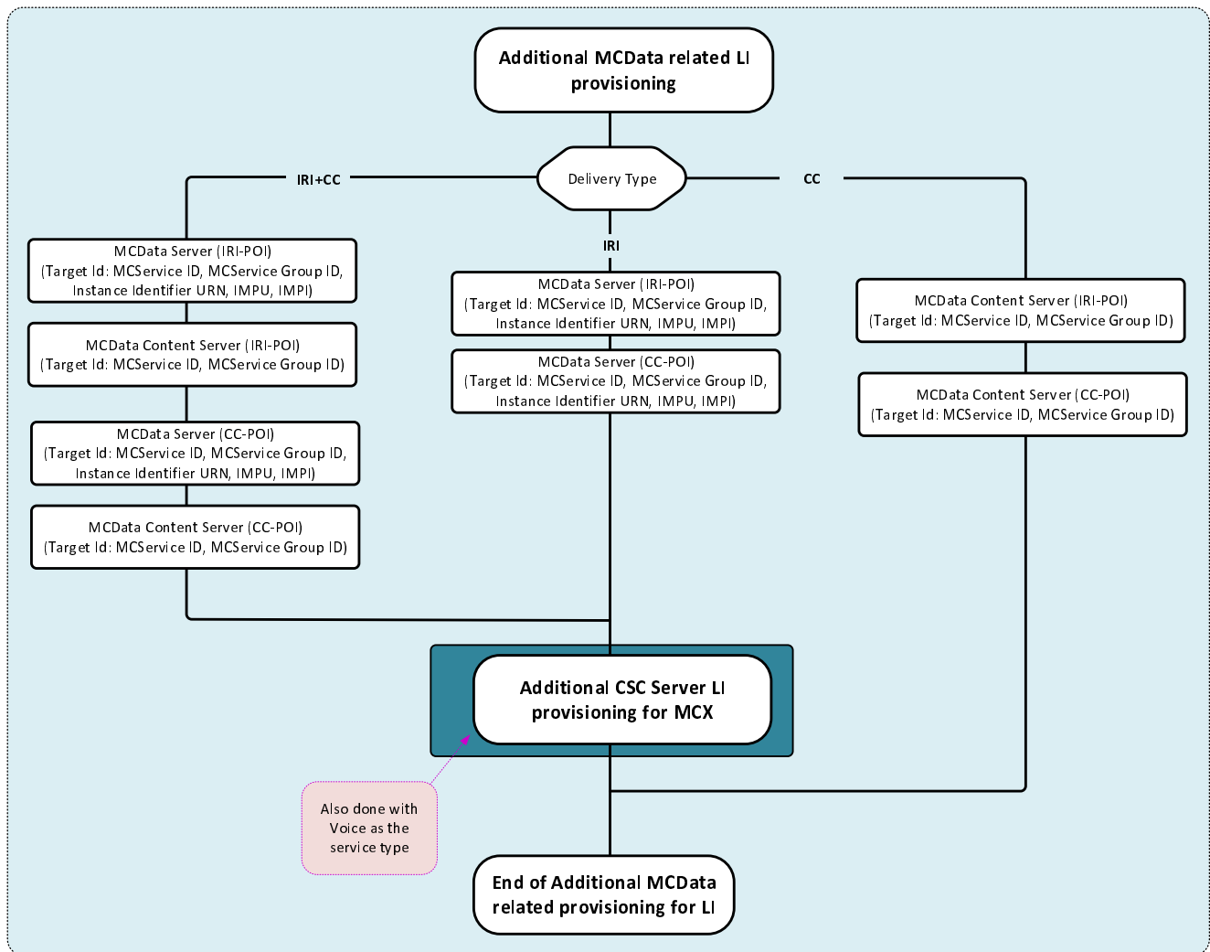
Figure 5.6.2.1-4: LIPF logic for MCDData related LI provisioning
