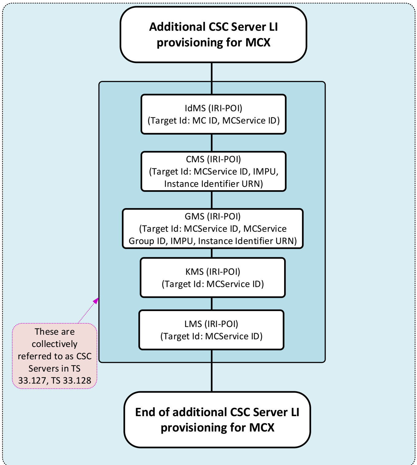
Figure 5.5.4.1-9: LIPF logic for additional CSC Server LI provisioning for MCX
