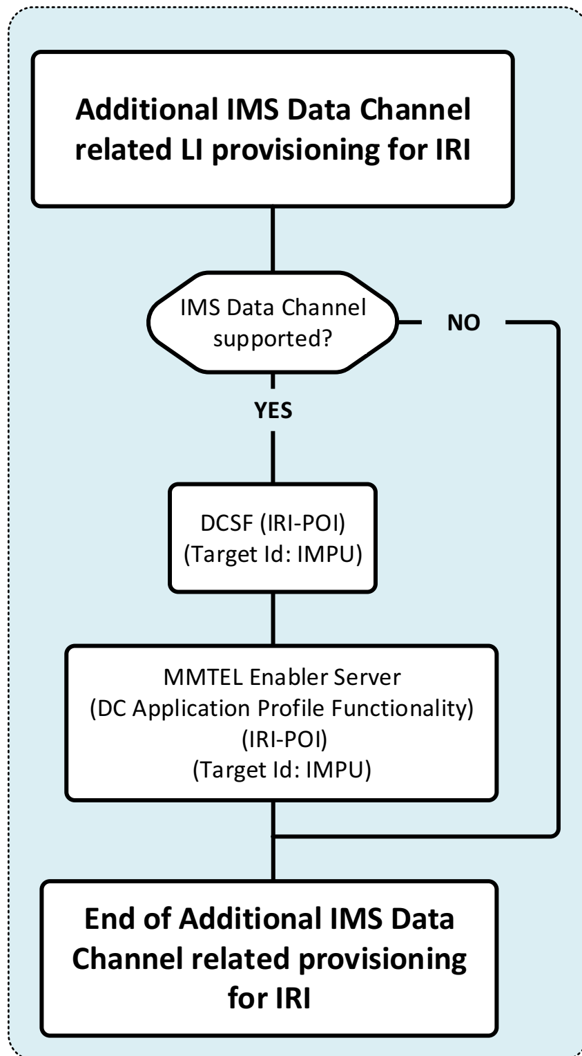
Figure 5.5.4.1-6: LIPF logic for additional IMS Data Channel related LI provisioning for IRI
