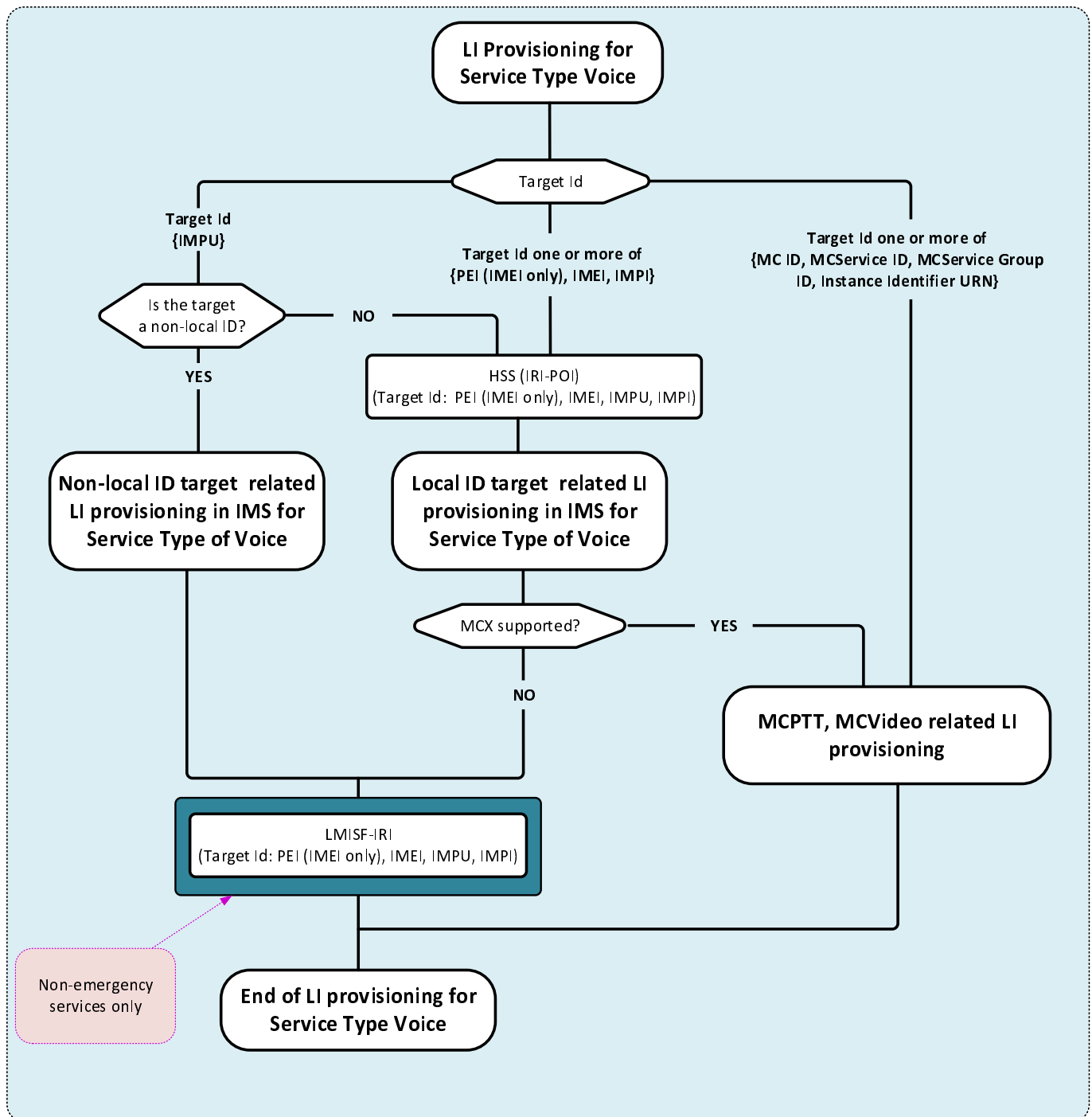
Figure 5.5.3-1: Top level view of LIPF logic for service type of Voice
