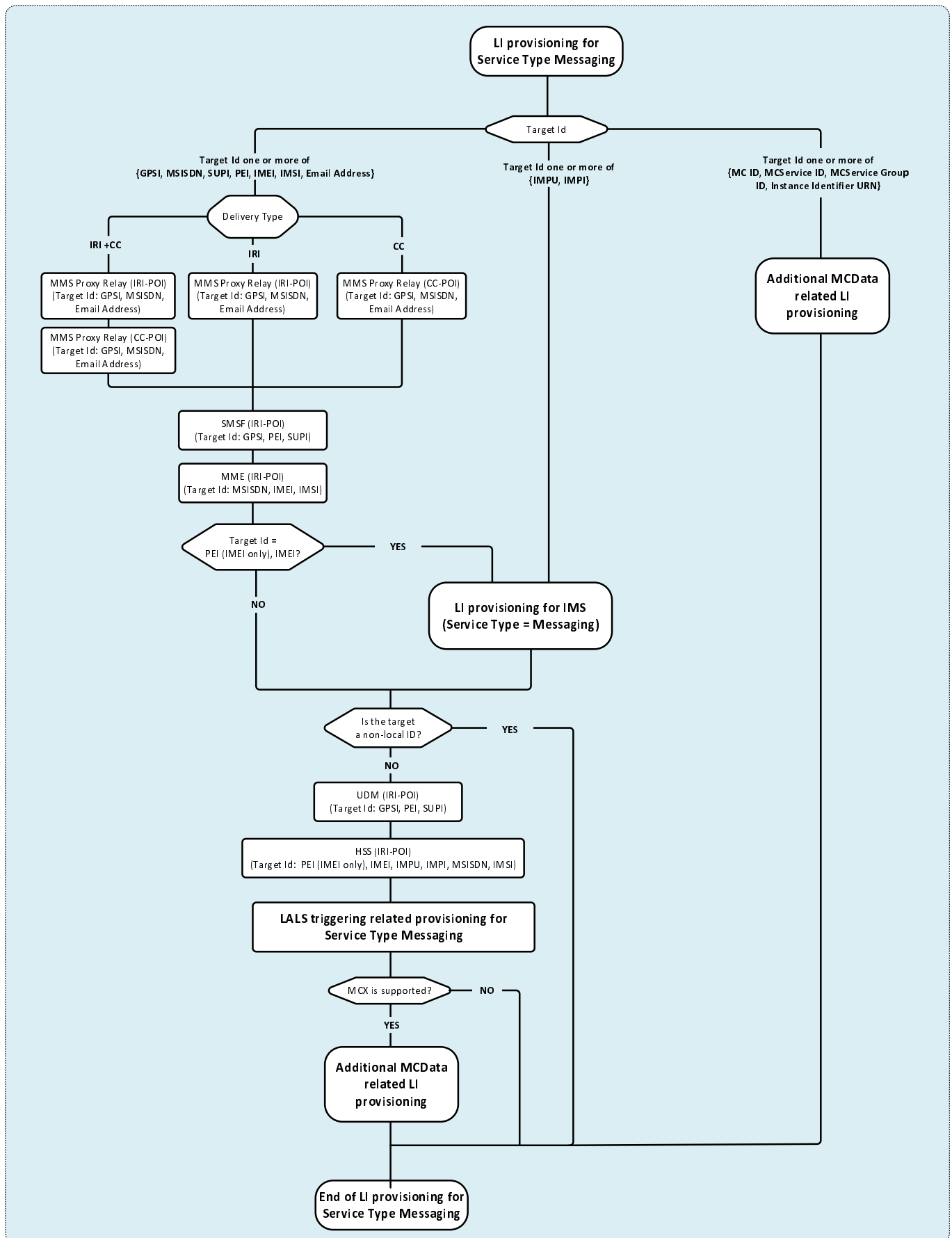
Figure 5.6.2.1-1: Top-level view of LIPF logic for service type of Messaging
