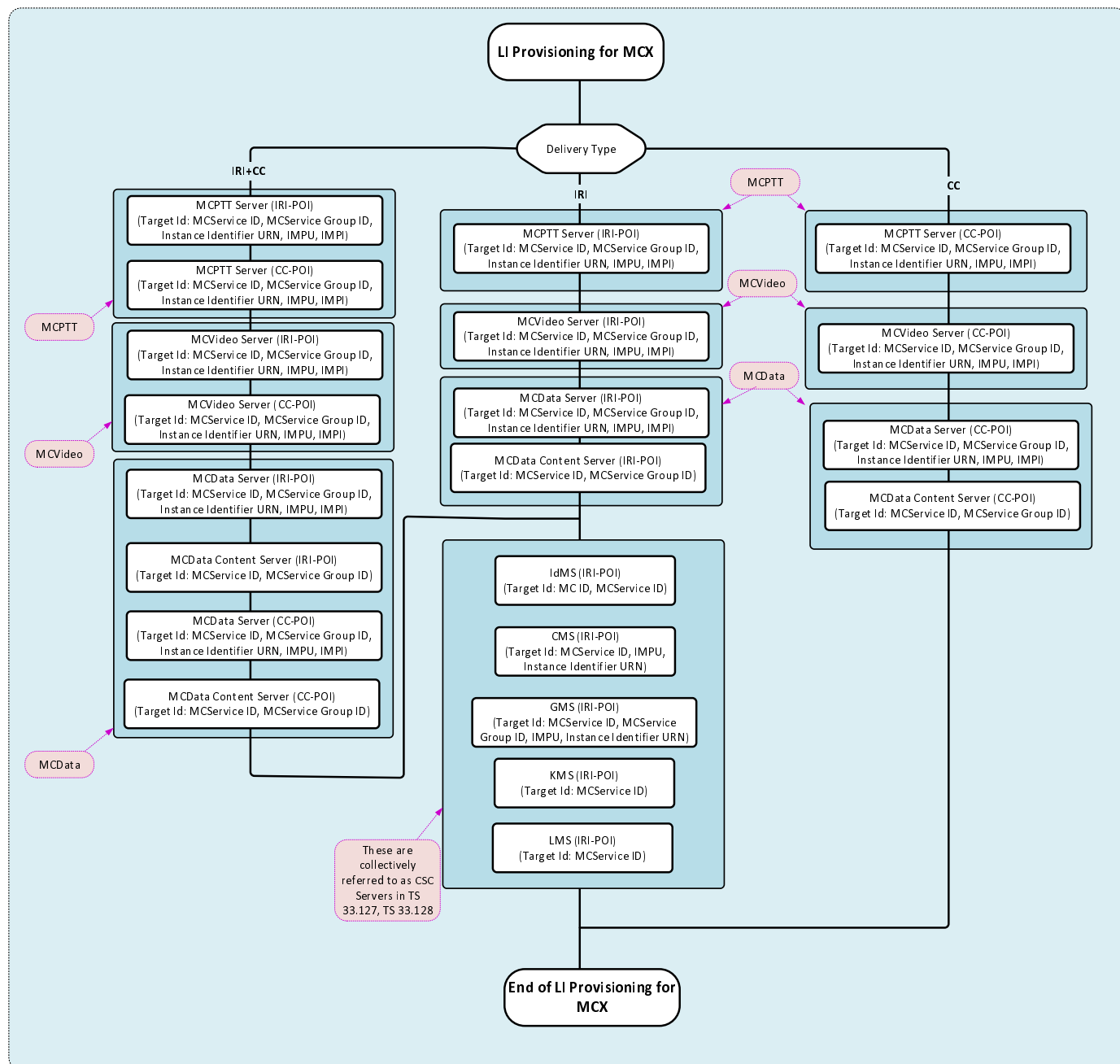
Figure 5.12.2-1: LIPF logic the provisioning of IRI-POI, CC-POI in MCX Servers and IRI-POI in CSC Servers
