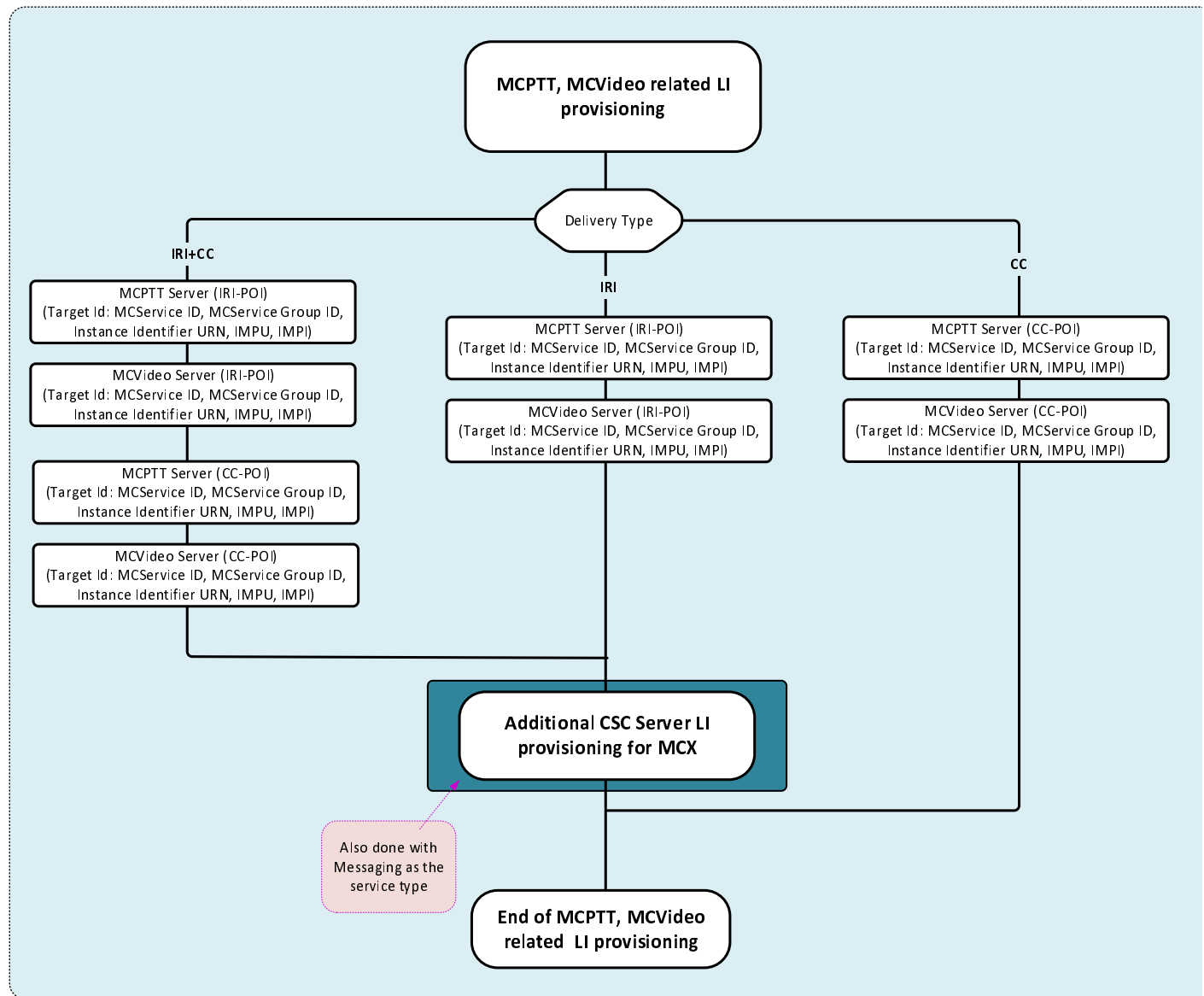
Figure 5.5.4.1-8: LIPF logic for MCPTT and MCVideo related LI provisioning
