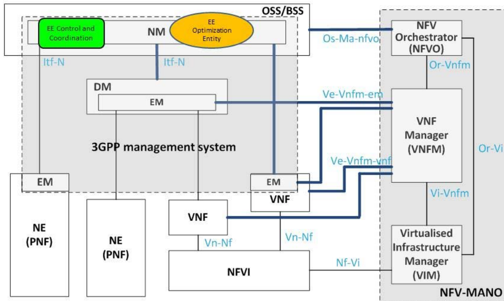
Figure 7.2.1.1: NM-centralised architecture
