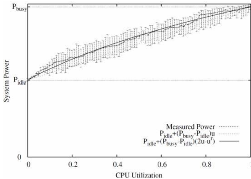
Figure 6.1: Power consumption of a server
