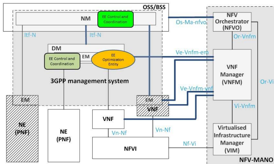
Figure 7.2.2.1: EM-centralised architecture
