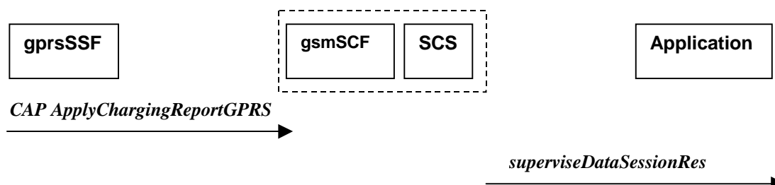
Figure 4-12: Call Flow for superviseDataSessionRes
