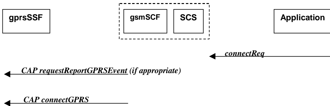
Figure 4-7: Call Flow for connectReq
