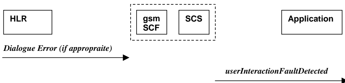
Figure 4-10: Call Flow for userInteractionFaultDetected (scenario 1)
