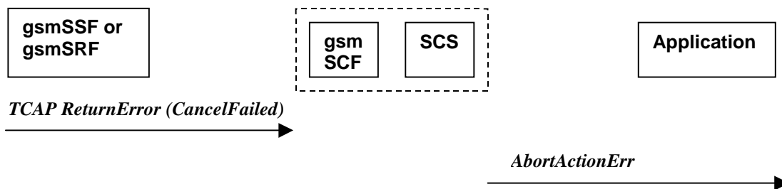
Figure 4-26: Call Flow for abortActionErr
