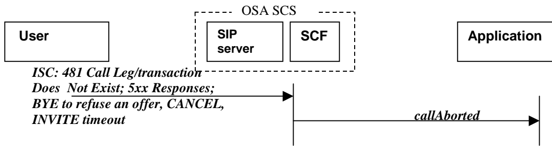
Figure 5-11: Call flow for callAborted()
