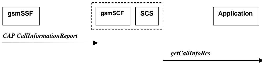
Figure 4-16: Call Flow for getCallInfoRes
