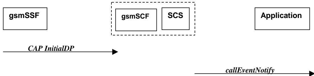
Figure 4-9: Call Flow for callEventNotify
