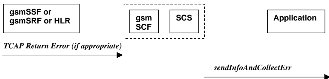
Figure 7-20: Call Flow for sendInfoAndCollectErr
