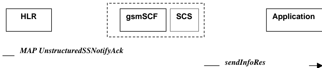
Figure 7-12: Call Flow for sendInfoRes (scenario 1)
