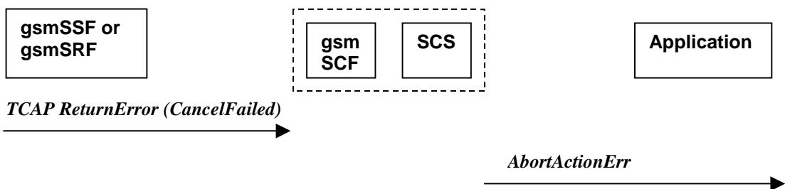
Figure 7-24: Call Flow for abortActionErr
