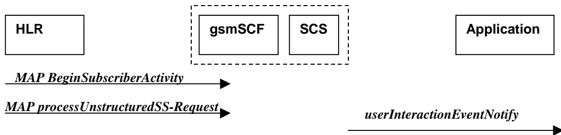
Figure 7-5: Call Flow for userInteractionEventNotify
