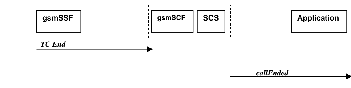
Figure 6-23: Call Flow for callEnded
