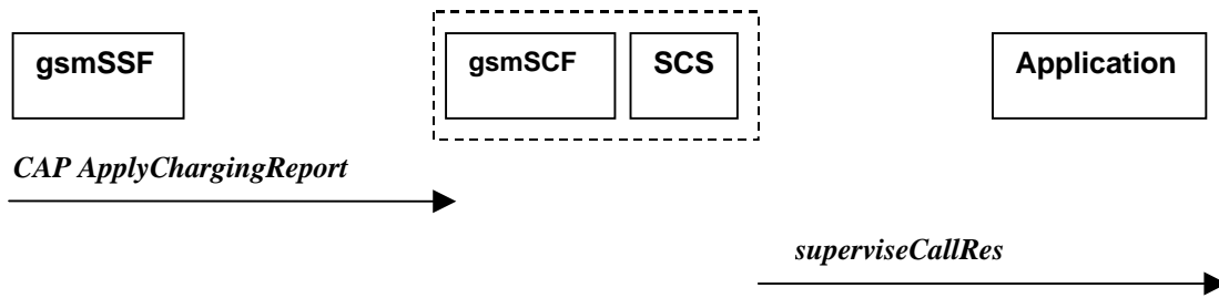
Figure 6-18: Call Flow for superviseCallRes
