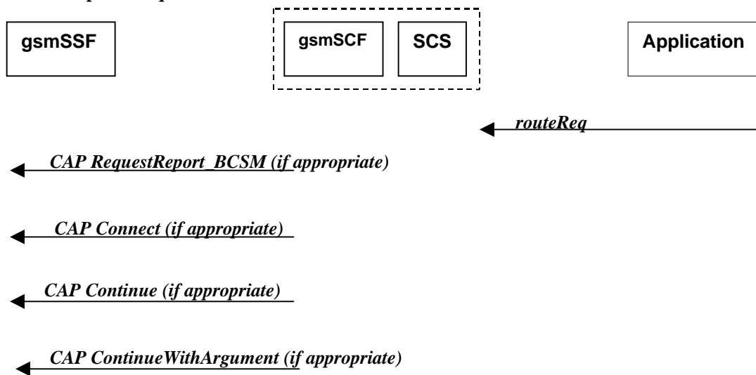
Figure 6-9: Call Flow for routeReq
