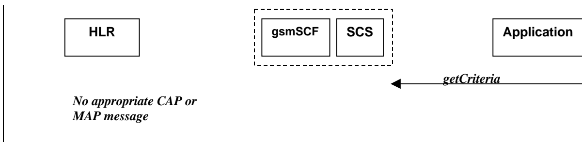
Figure 6-4: Call Flow for getCriteria
