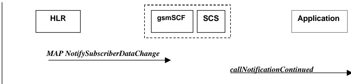
Figure 6-6: Call Flow for callNotificationContinued
