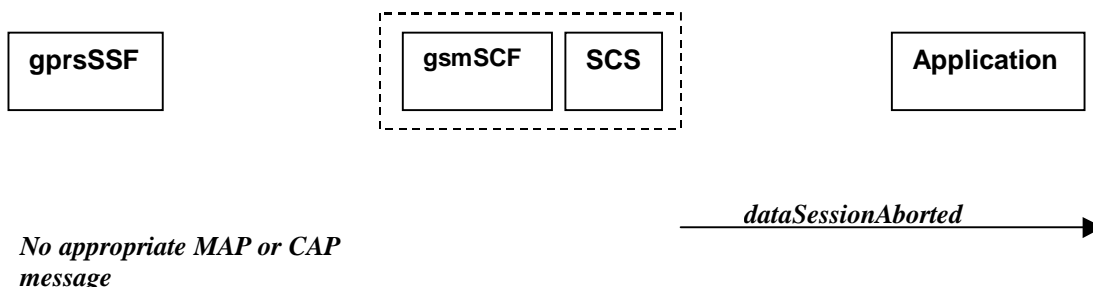
Figure 13-4: Call Flow for dataSessionAborted
