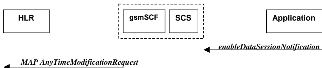
Figure 13-1: Call Flow for enableDataSessionNotification
