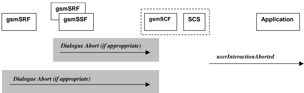
Figure 7-7: Call Flow for userInteractionAborted (scenario 2)
