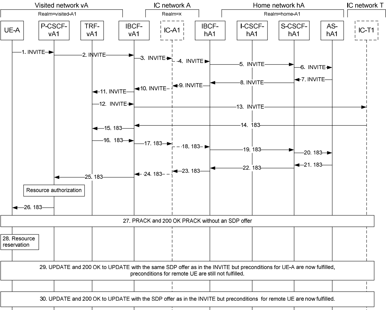
Figure 5.4.2-1: MOC with loopback
