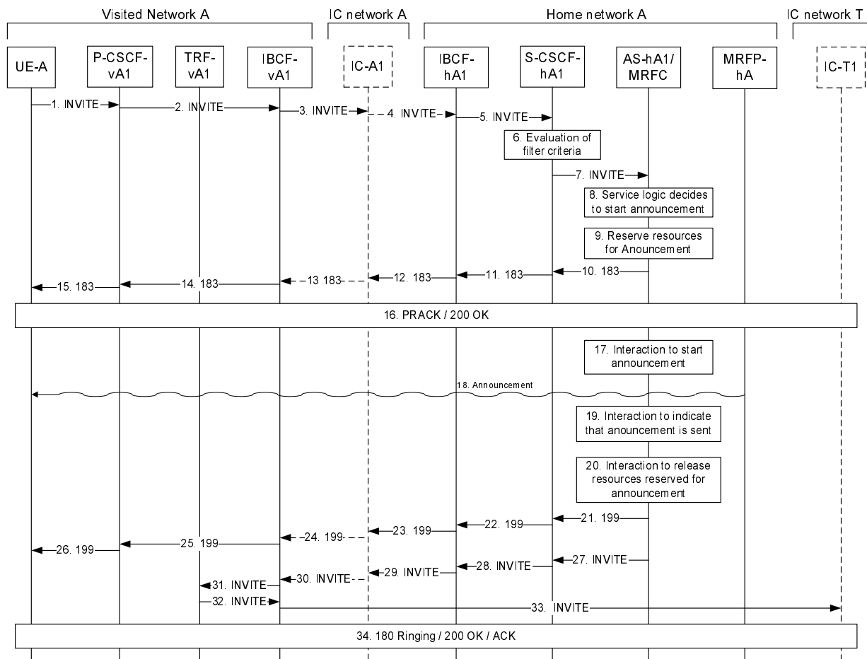
Figure 5.10.2-1: Announcement started during the establishment of a communication
