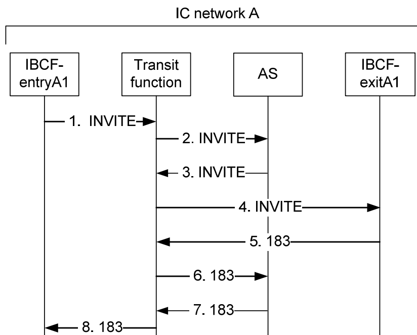
Figure 4.3.1.5-1: IOI exchange for IMS roaming transit
