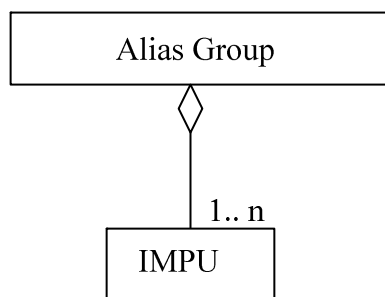
Figure 11.3-6 Information model for Alias Group
