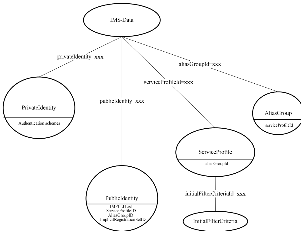
Figure 11.2.4-1: DIT Structure for IMS-Data with Alternative D
