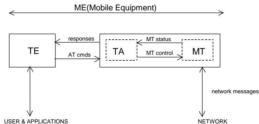
Figure 1: The 3GPP terminal model
