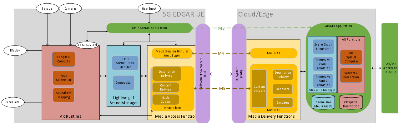
Figure 4.2.2.3-1: Functional structure for Type 2: 5G EDGE-Dependent AR (EDGAR) UE
