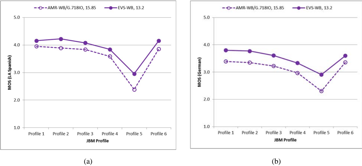
Figure 9: EVS WB vs AMR-WB – Speech - TS 26.114 Delay & Error Profiles
