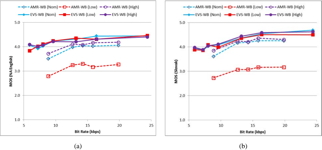
Figure 7: EVS WB vs AMR-WB – Speech – Clean Channel & Levels
