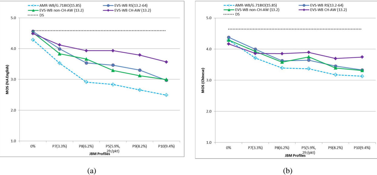
Figure 10: EVS WB vs AMR-WB – Speech – New EVS JBM Delay & Error Profiles
