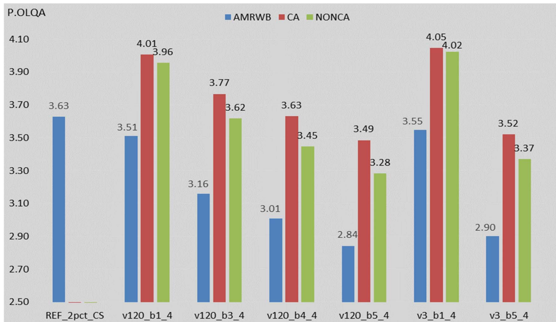
Figure 5.1.1.6.3.3-3: P.OLQA scores for Case 2 – Superswideband Speech
