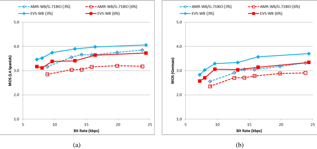
Figure 8: EVS WB vs AMR-WB – Speech - Random Frame Erasures
