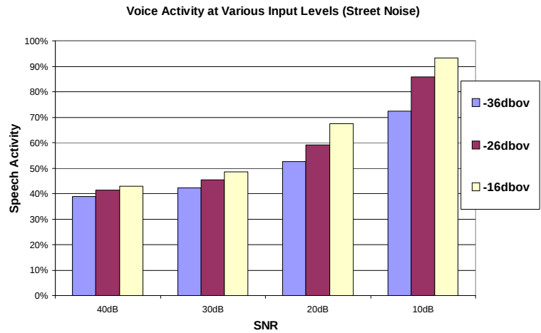
Figure 29.5: Voice Activity for different input levels (street noise)
