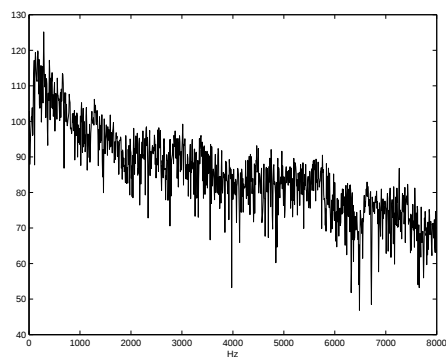
a) Frequency spectrum of the "car" noise
