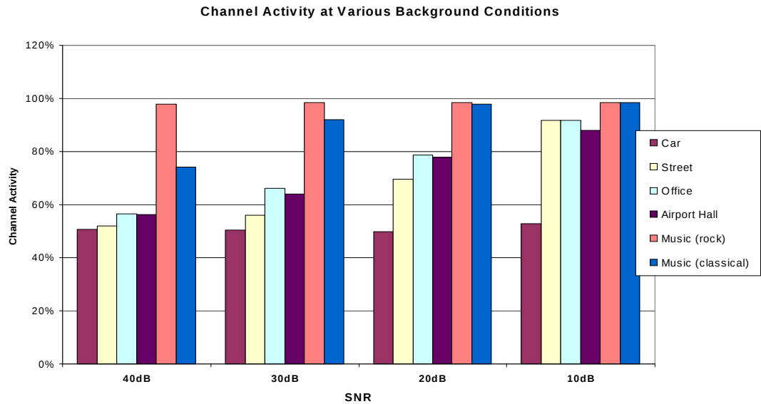
Figure 29.4: Channel Activity for different background conditions, input speech level = -26\text{dBov} (for clean speech; channel activity = 51 %)
