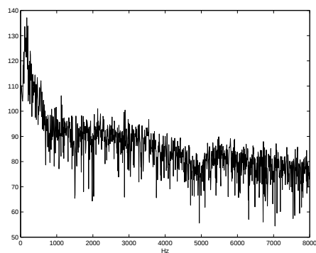
b) Frequency spectrum of the "cafeteria" noise
