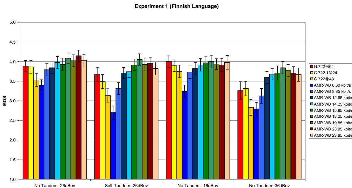
Figure 8.1: Experiment 1, testing Tandeming and input levels with Finnish language
