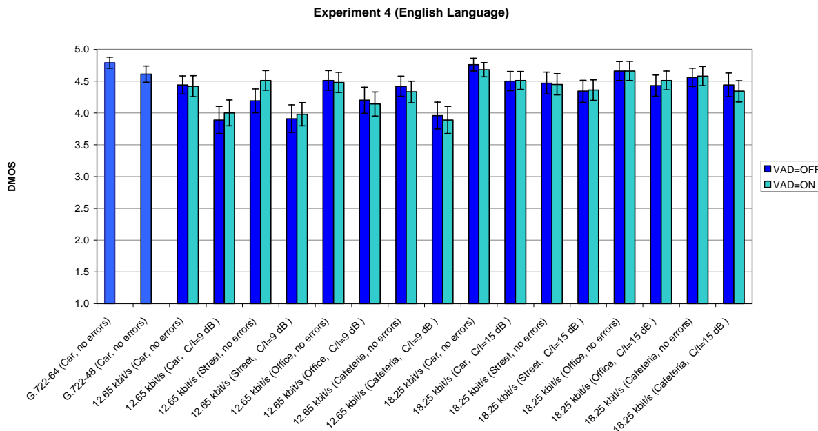
Figure 11.1: Experiment 4, testing VAD/DTX with English language
