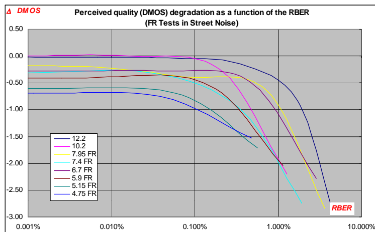
Figure D3c: Quality Degradation function of RBER (FR Test Results)
