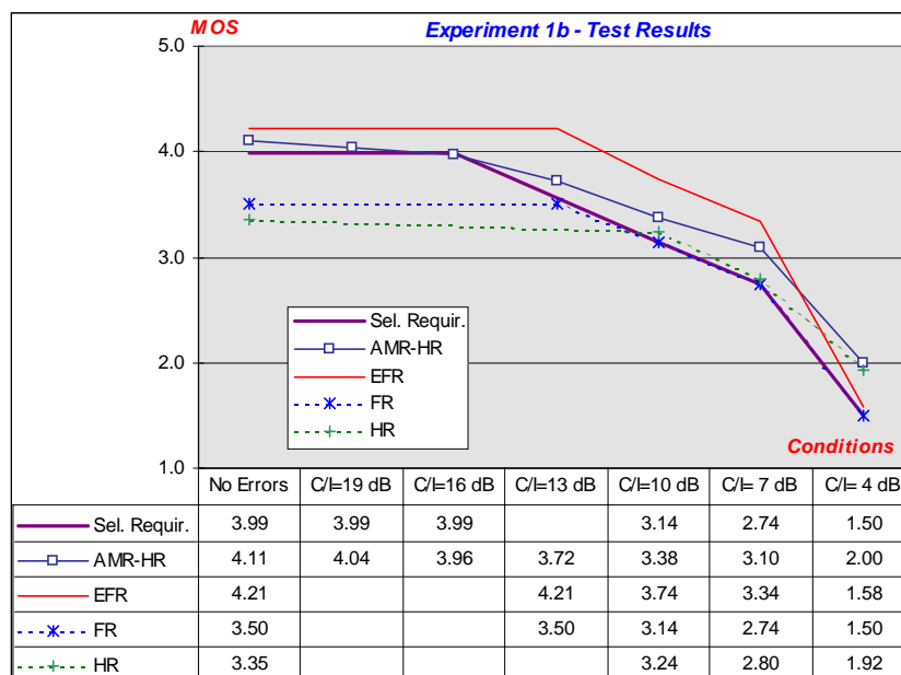
Figure 5.3: AMR half rate/clean speech performances curve (Best AMR Codec vs. EFR vs. GSM FR vs. GSM HR vs. Performance Requirements)
