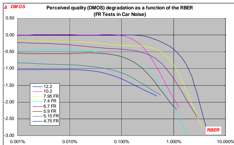
Figure D2c: Quality Degradation function of RBER (FR Test Results)
