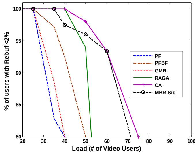
Figure 8.5: CDF of Re-buffering Outage
