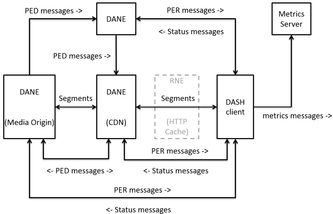
Figure 4.2: SAND reference architecture (taken from ISO/IEC 23009-5 [2])
