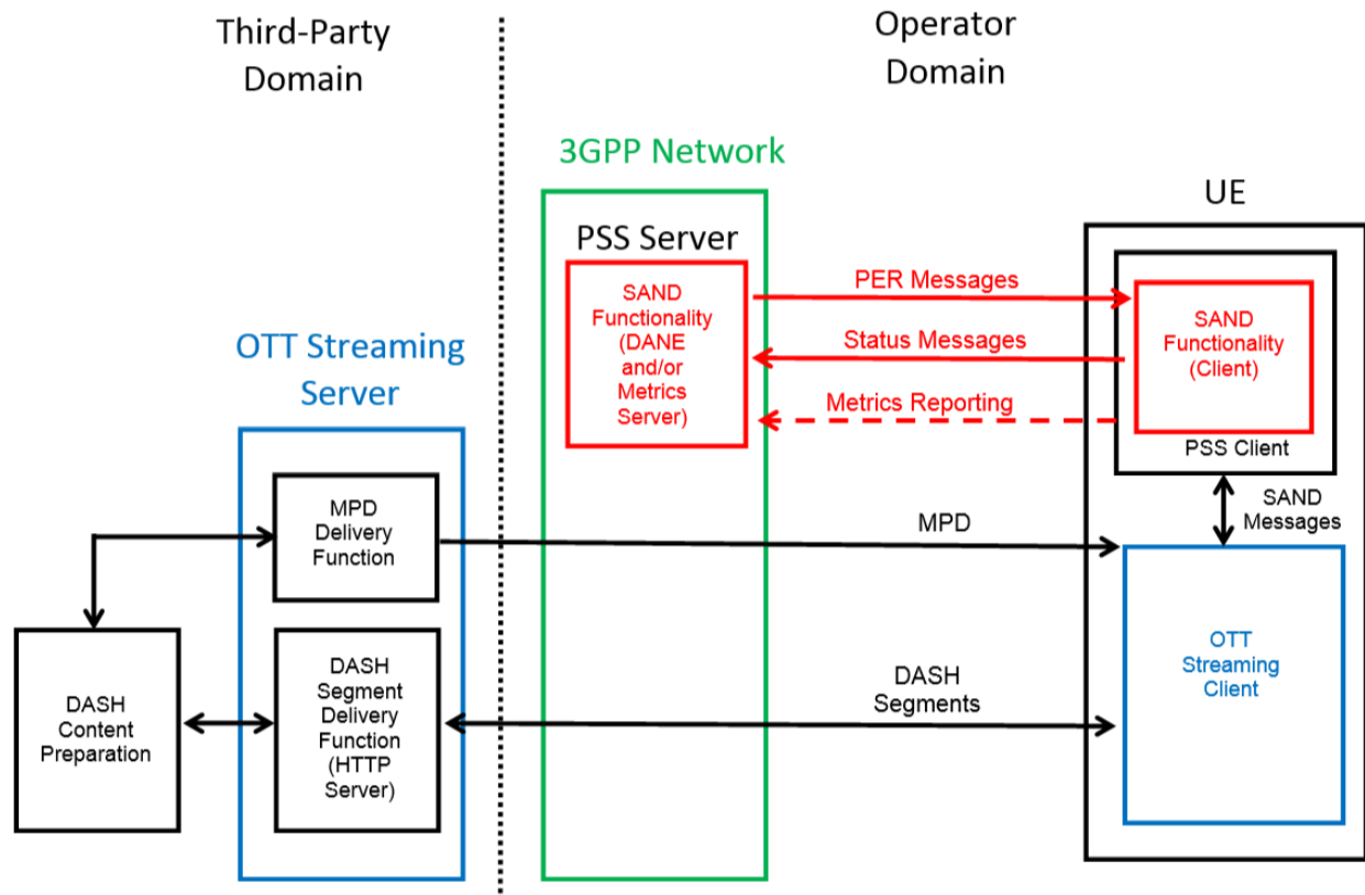
Figure 5.4: Alternative SAND architecture for OTT Streaming Services
