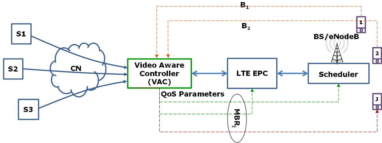
Figure 8.2: Video Aware QoS Signaling Architecture
