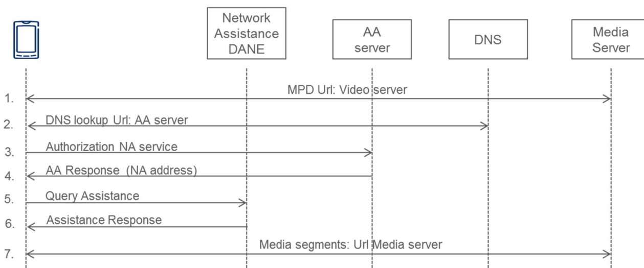
Figure 6.6. Sequence for Network Assistance between the media client and the network
