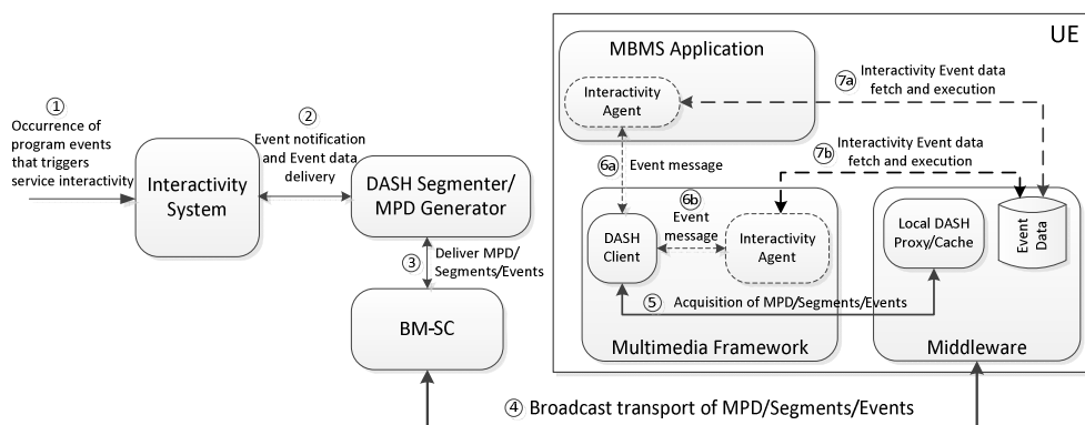
Figure 5.2: Service Interactivity Architecture for Broadcast DASH
