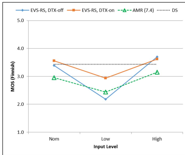
Figure 9.9: Experiment N1, testing EVS-NB clean speech at various input levels with Finnish language
