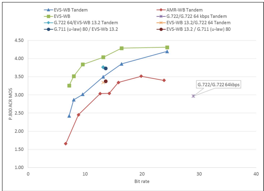
Figure 10.30: Experiment W5, testing EVS-WB clean speech with Danish language
