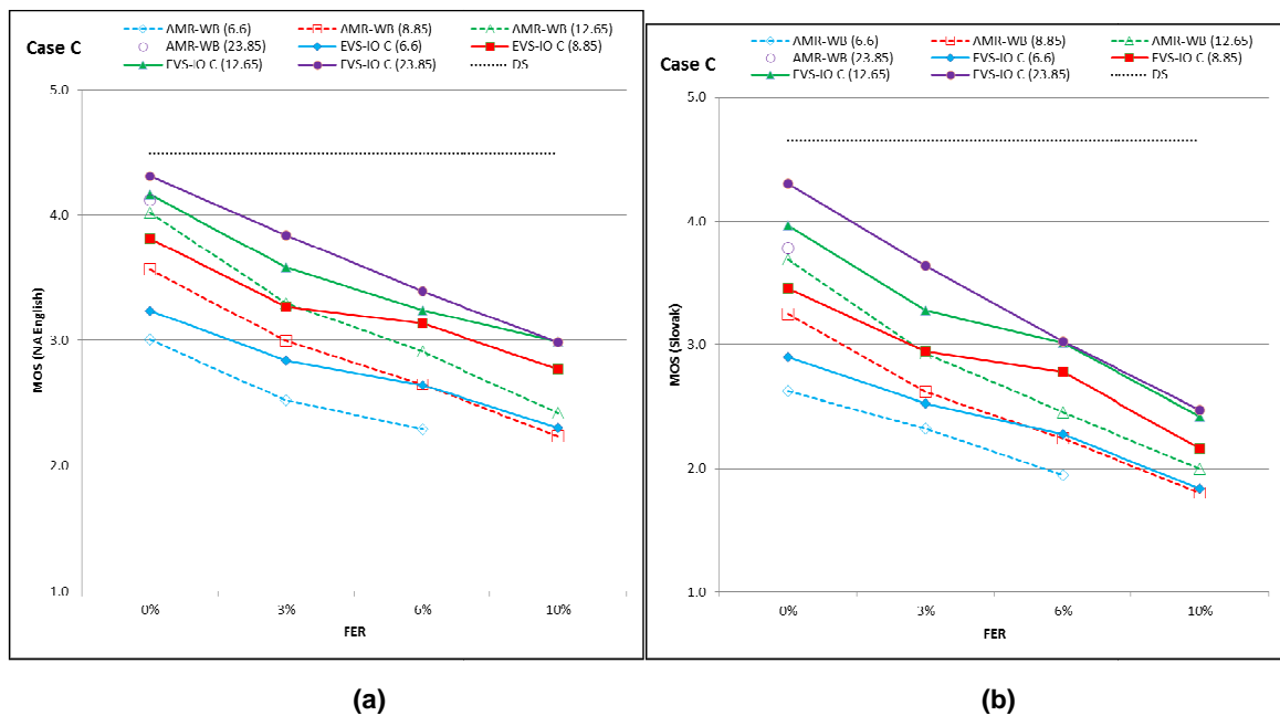
Figure 10.24: Experiment W3, testing EVS-WB clean speech in EVS AMR-WB IO Case C (a) with North American English language and (b) with Slovak language
