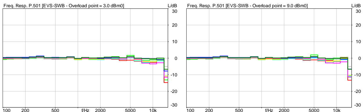
Figure13.9: Frequency response EVS SWB in 1/3^{\text{rd}} Oct. for different overload points with P.501 speech signals
