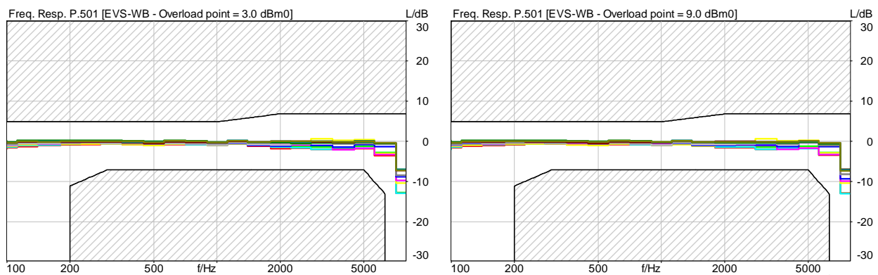
Figure 13.7: Frequency response EVS WB in 1/3^{\text{rd}} Oct. for different overload points with P.501 speech signals
