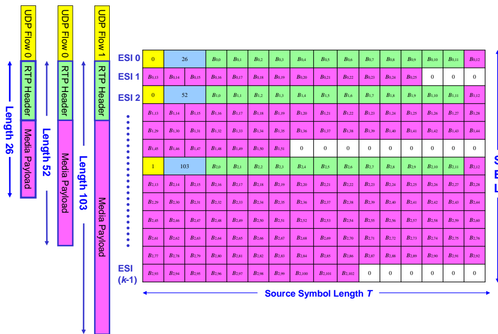
Figure 2: MBMS Streaming Framework
