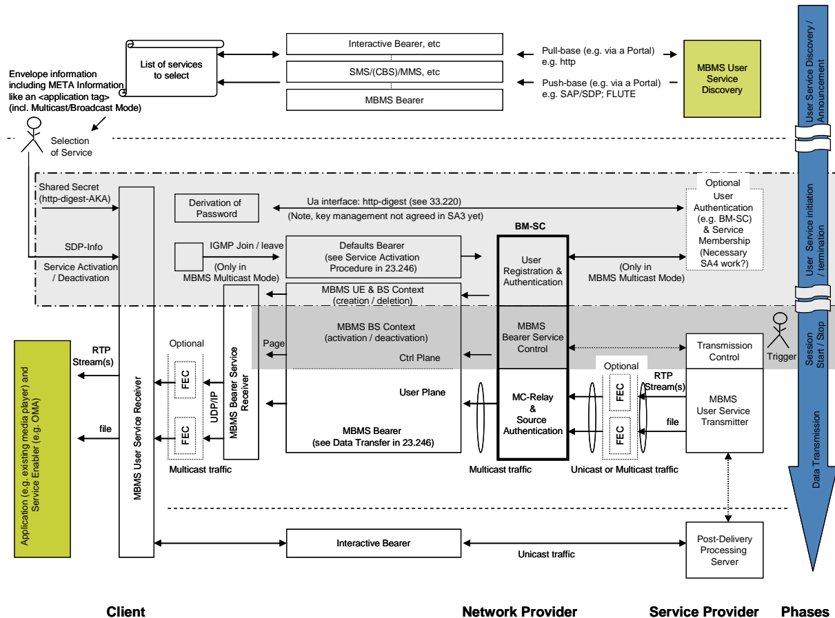
Figure 2: MBMS system overview
