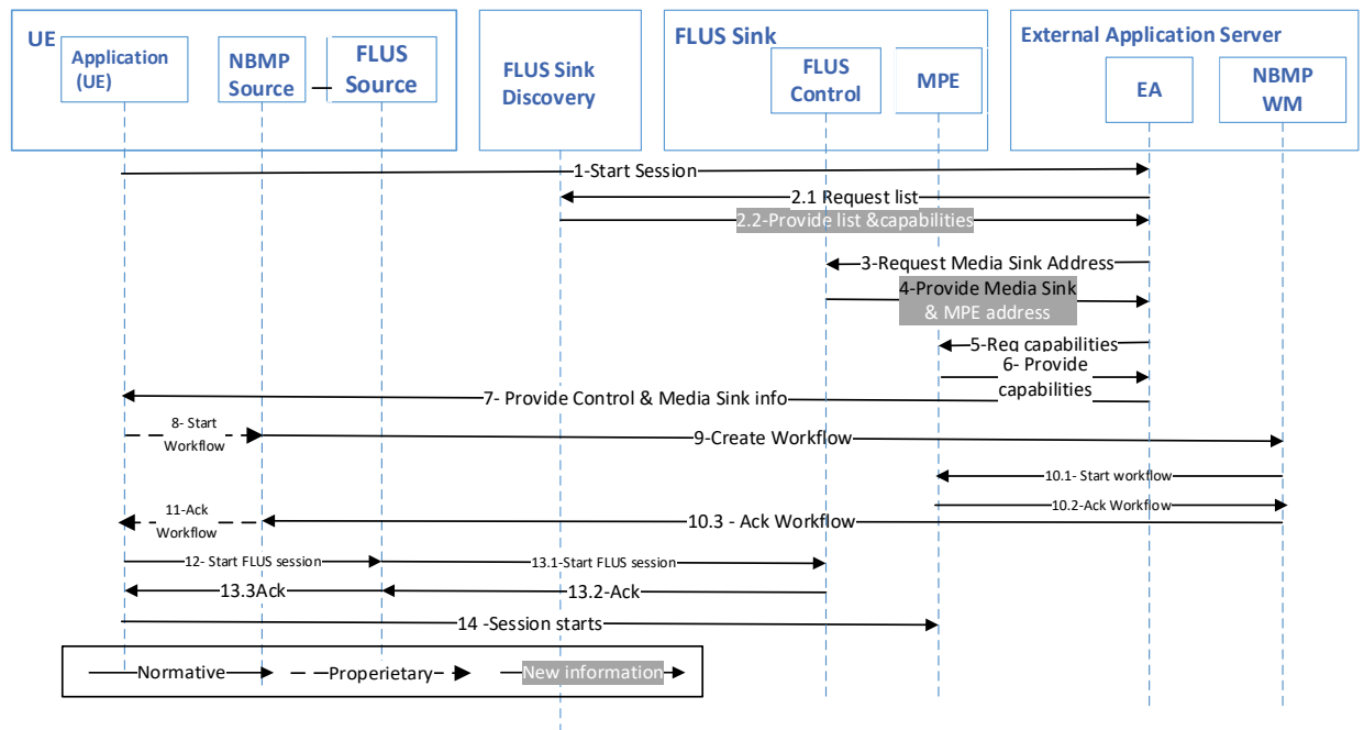
Figure 8.4.6.2.2-1: Call flow for NBMP Client in the UA, NBMP Workflow Manager in the Application Server and MPE in Sink through N3
