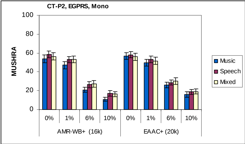
Figure 4: Audio content for audio codecs across PLR (EGPRS mono mode) (Bit-rates given are gross rates including packetization overhead)
