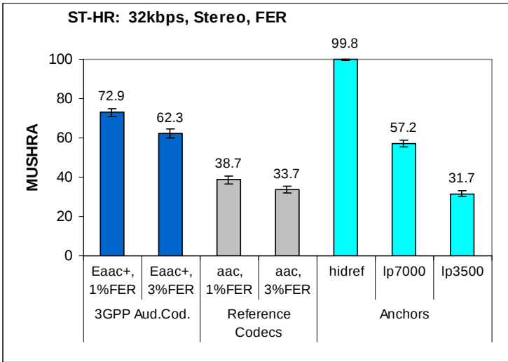
Figure 22: MUSHRA results at 32 kbps with 3 % errors (stereo)
