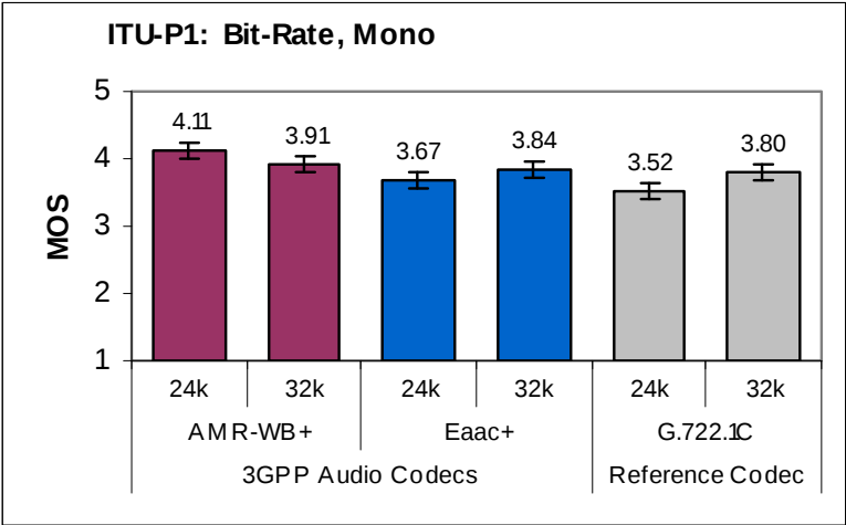
Figure A.3: MOS for audio codecs at bit-rates of 24 and 32 kbps (speech-only)
