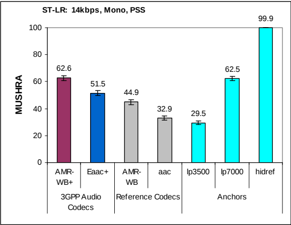
Figure 12: Results at 14 kbps for PSS (mono)
