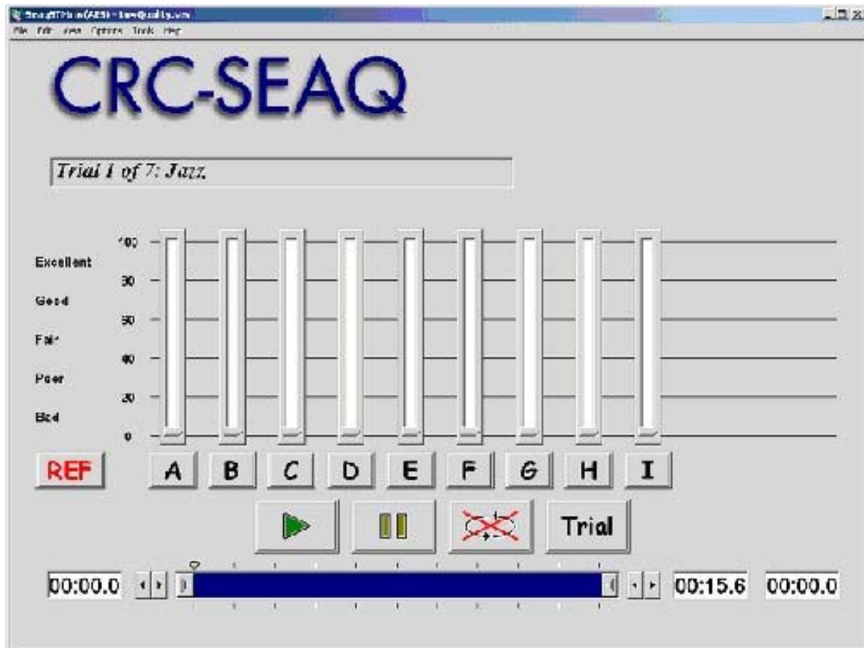
Figure 47: MUSHRA software
