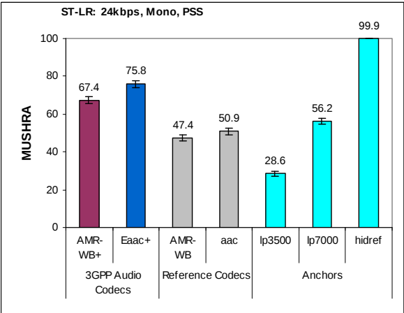
Figure 13: Results at 24 kbps for PSS (mono)
